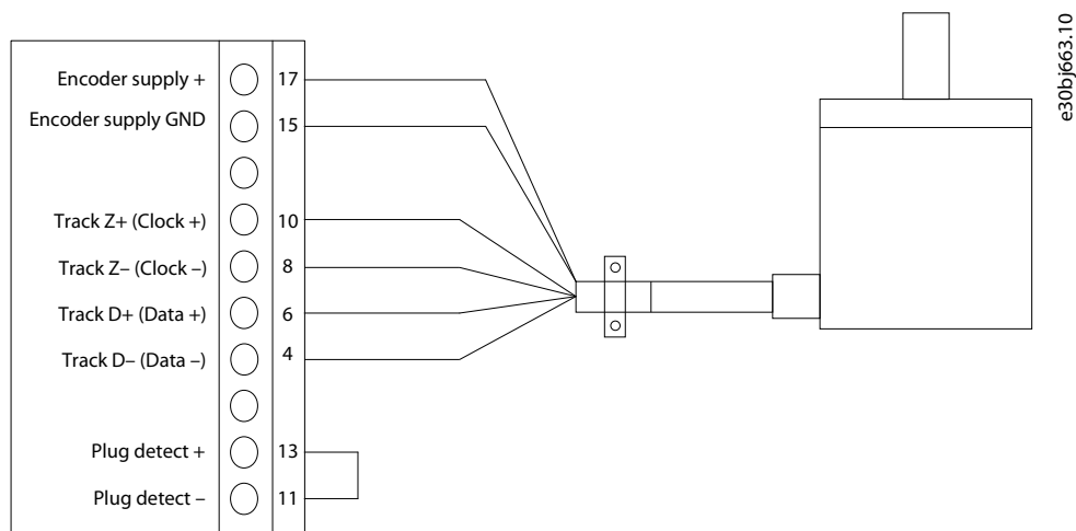
Illustration 11: Wiring Configuration for 2-Track BiSS Encoder
