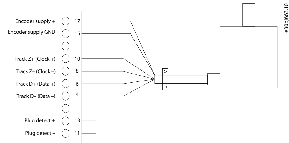
Illustration 10: Wiring Configuration for 2-Track EnDat Encoder
