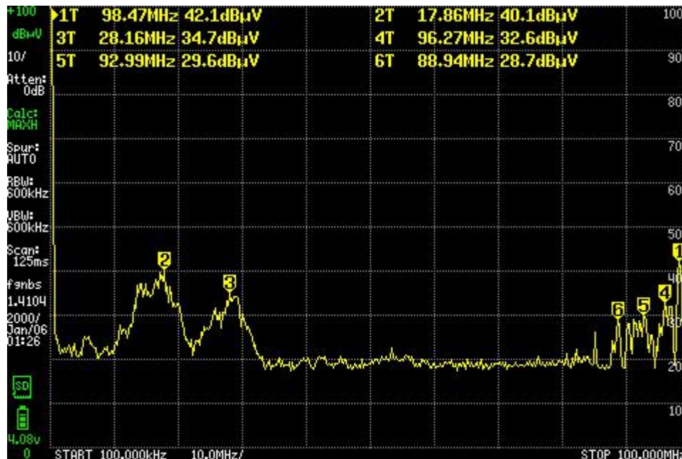
[图 2.5] This diagram shows the SA5, with an external telescopic antenna, to test the EMC emissions of a Tesla Model 3 while driving.
