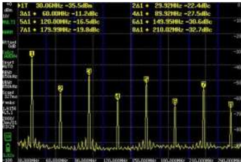
[图 2.6] This diagram shows the harmonic measurement function in the SA5's measurement menu to measure the harmonics of a 30MHz square wave signal.
