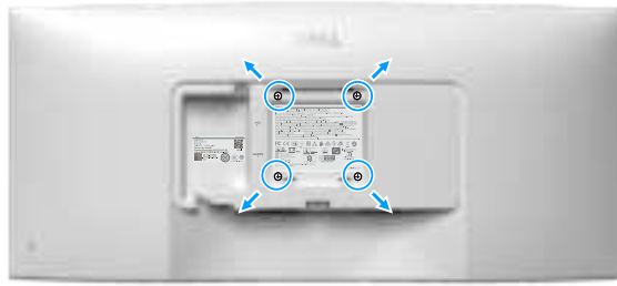
Figure 26. Wall mounting
