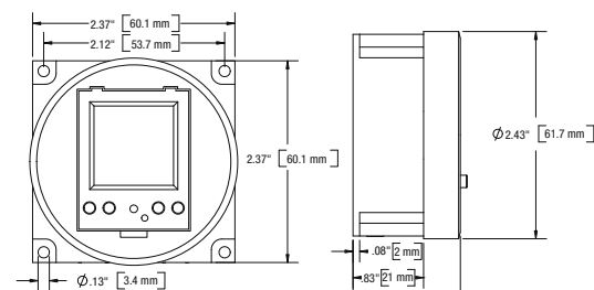
FM1D20 Flush Mount with Clear Dust Cover
