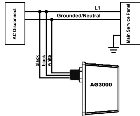
AG3000 Wiring Diagram - Type 2 120 VAC
