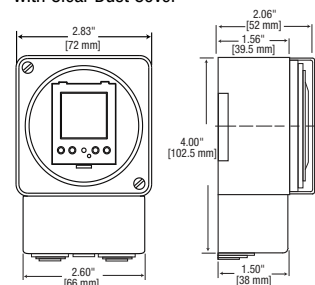
FM1D20A Surface/DIN Rail with Clear Dust Cover
