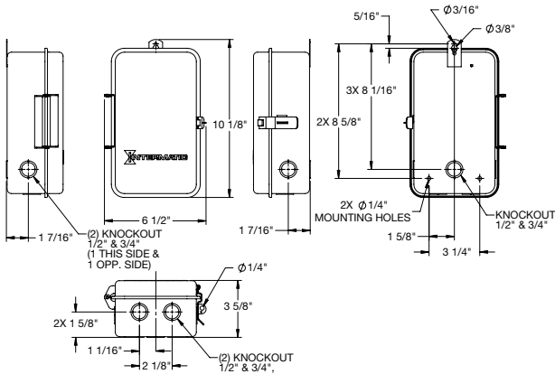
2T2485GA Dimensions
