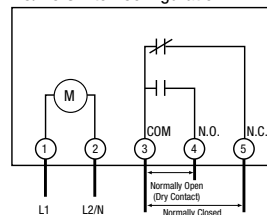
NO/NC Switch Configuration
