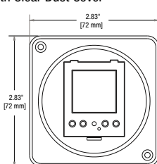
FM1D20E Flush Mount with Clear Dust Cover
