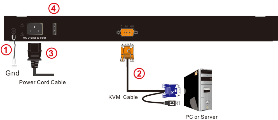
1-4 cable connection
