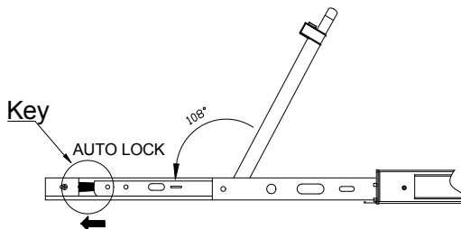
Figure 2-5 unlocking the slide rail
