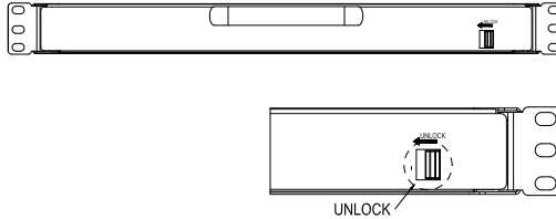
Figure 2-3 unlocking
