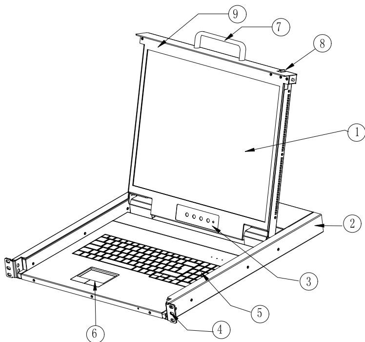
Figure 1-2 front view
