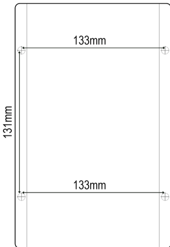
Figure 2 Mounting Diagram
