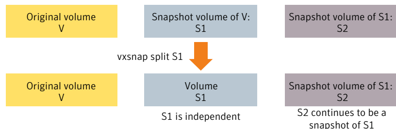
Figure 23-7 Splitting snapshots
