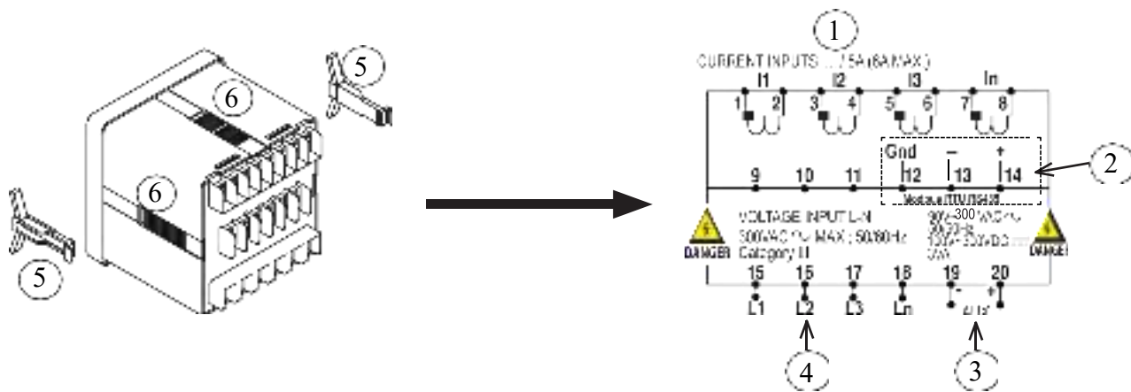
Figure 1: Parts of power meter
