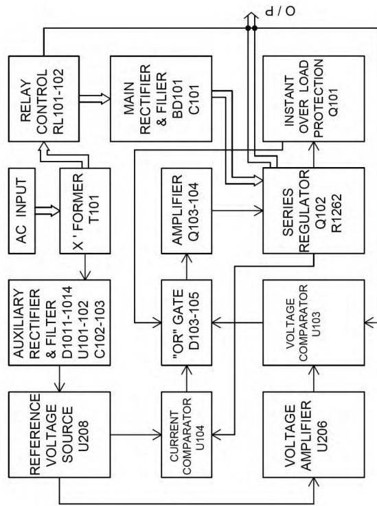
Block diagram
