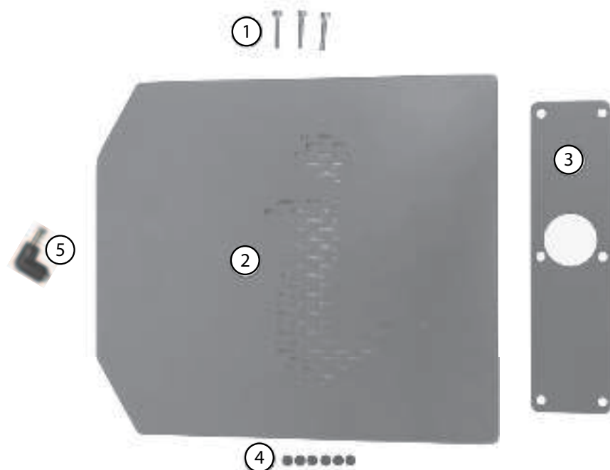
Figure 1. iDimension Plus Retrofit Kit Parts
