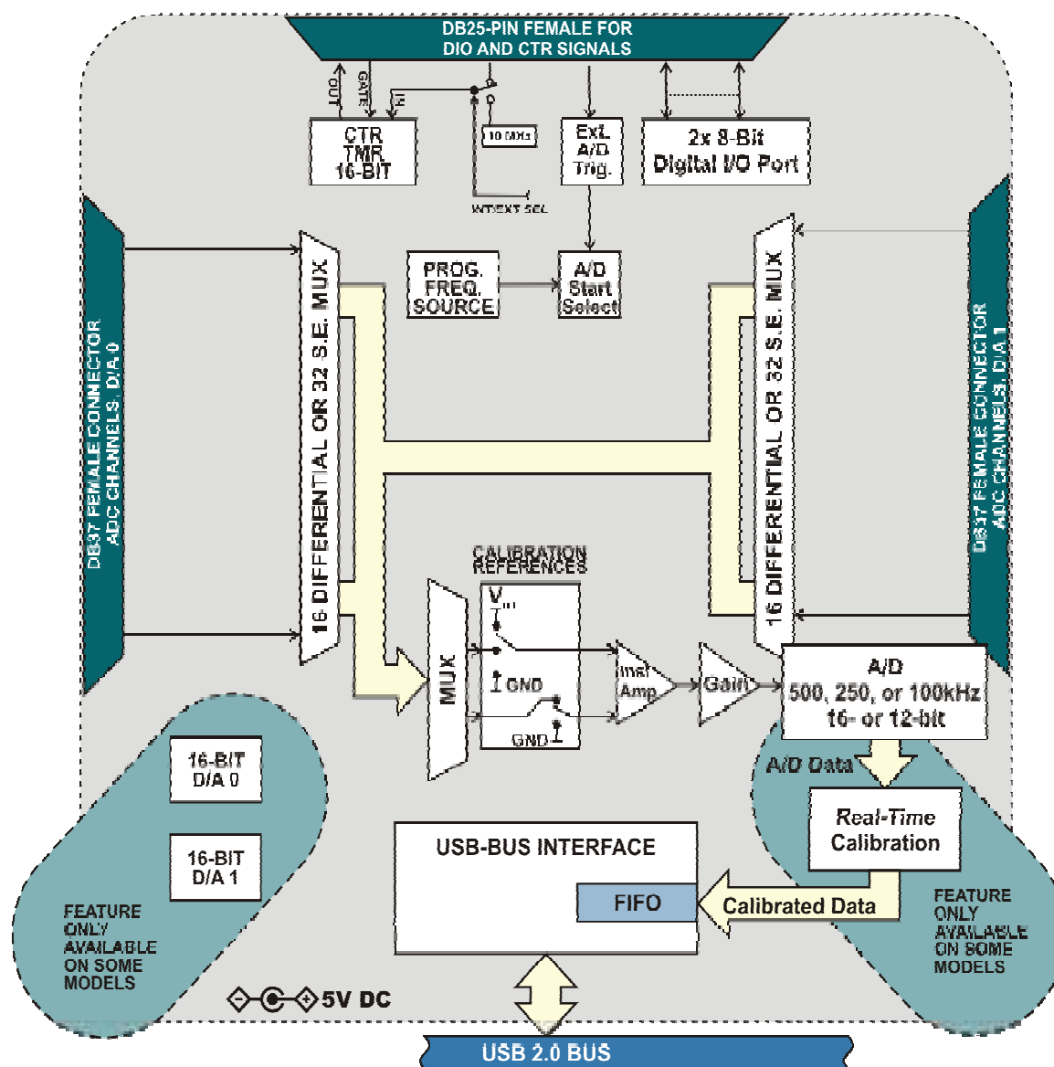
Figure 1-1: Block Diagram
