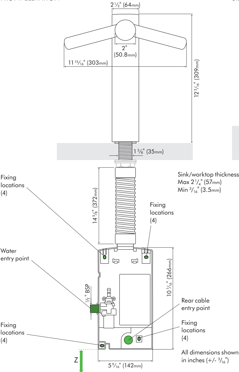
FRONT ELEVATION
