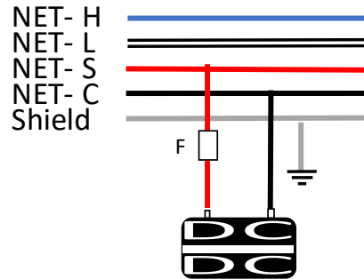
An isolated Power Supply
