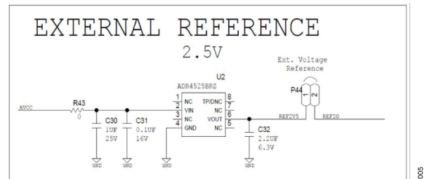
Figure 5. External Reference Connection
