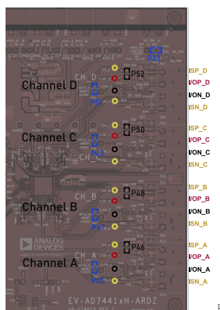
Figure 7. Output Channels
