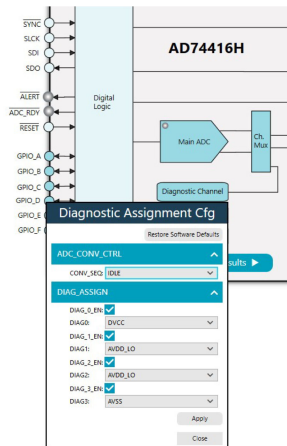
Figure 15. Assigning Diagnostic
