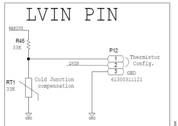
Figure 6. LVIN PIN Connection
