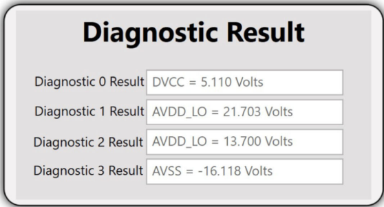
Figure 17. Diagnostics Measurements
