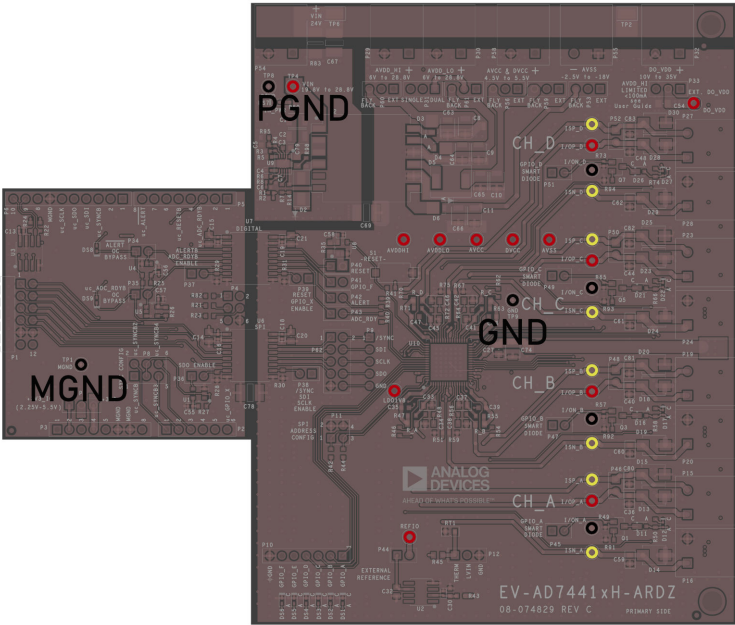
Figure 8. EVAL-AD74416H-ARDZ Test Points
