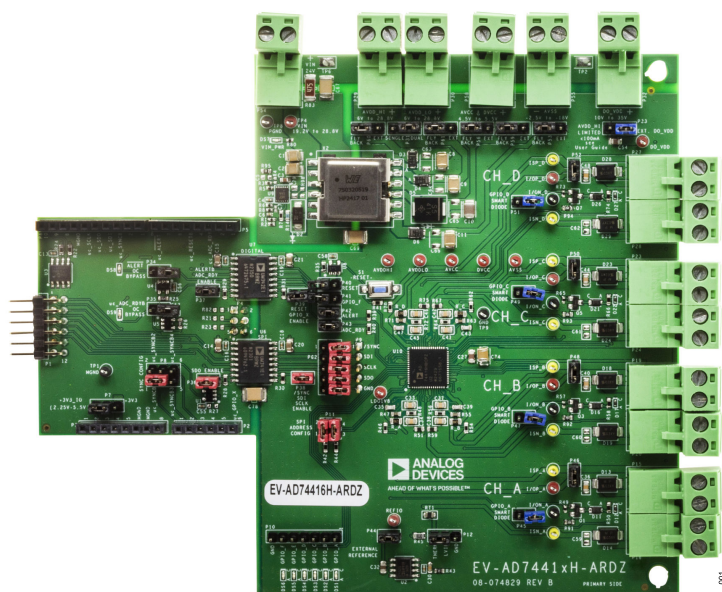
Figure 1. EVAL-AD74416H-ARDZ Evaluation Board Photograph
