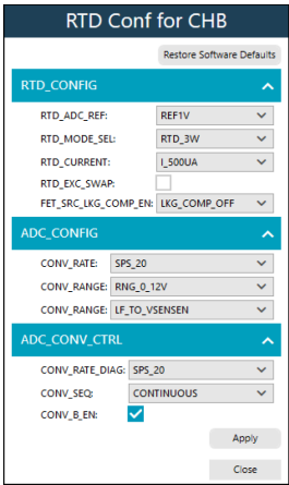
Figure 21. 3-Wire RTD Configuration to Measure Pt1000 at Channel B
