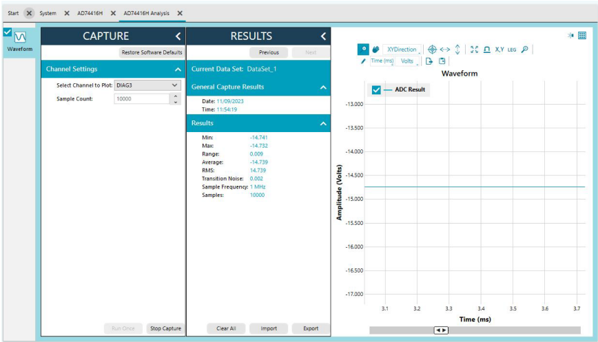
Figure 18. Analysis Window
