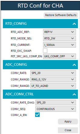
Figure 20. 2-Wire RTD Configuration to Measure Pt1000 at Channel A
