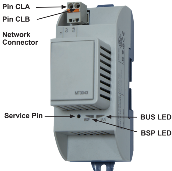
Figure 4: LONWORKS Communication Module - Main Features
