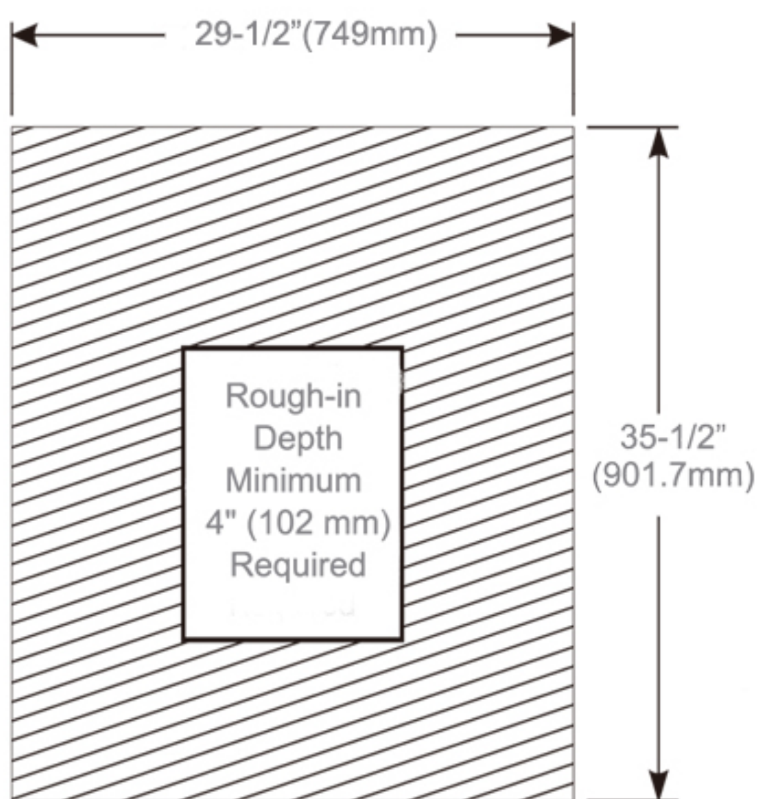
Rough-in Dimensions
