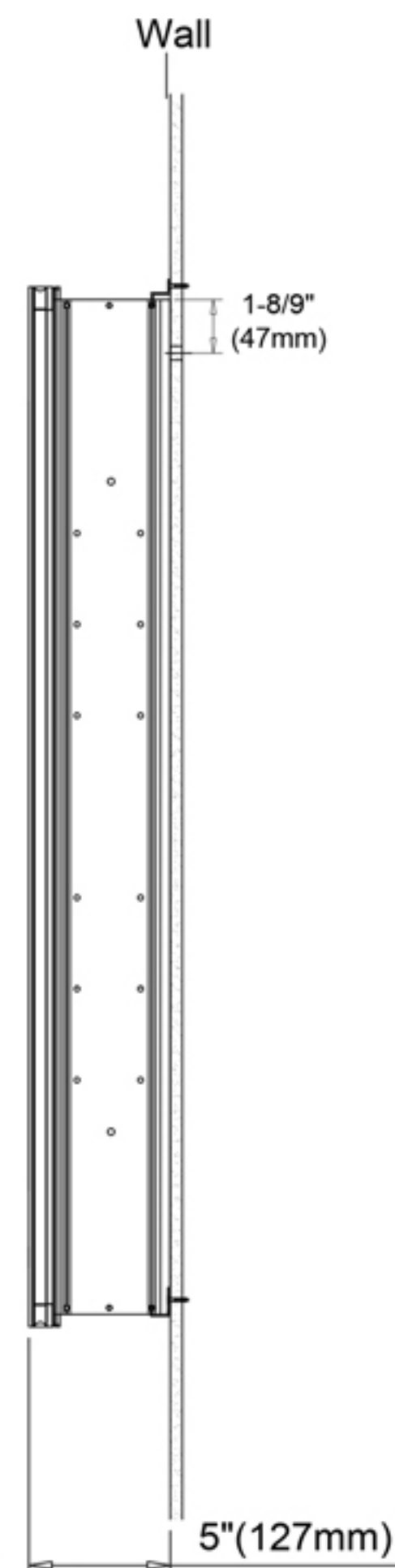
Surface Mount
