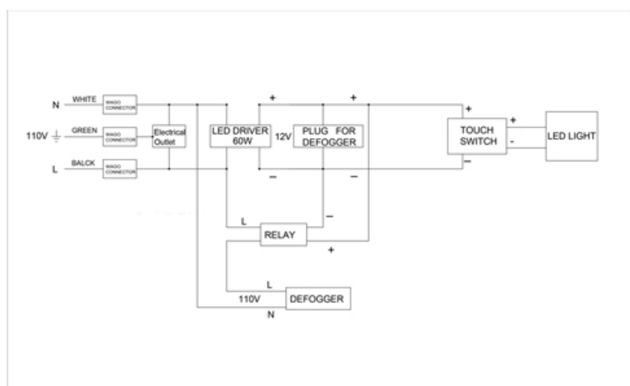
Circuit Diagram
