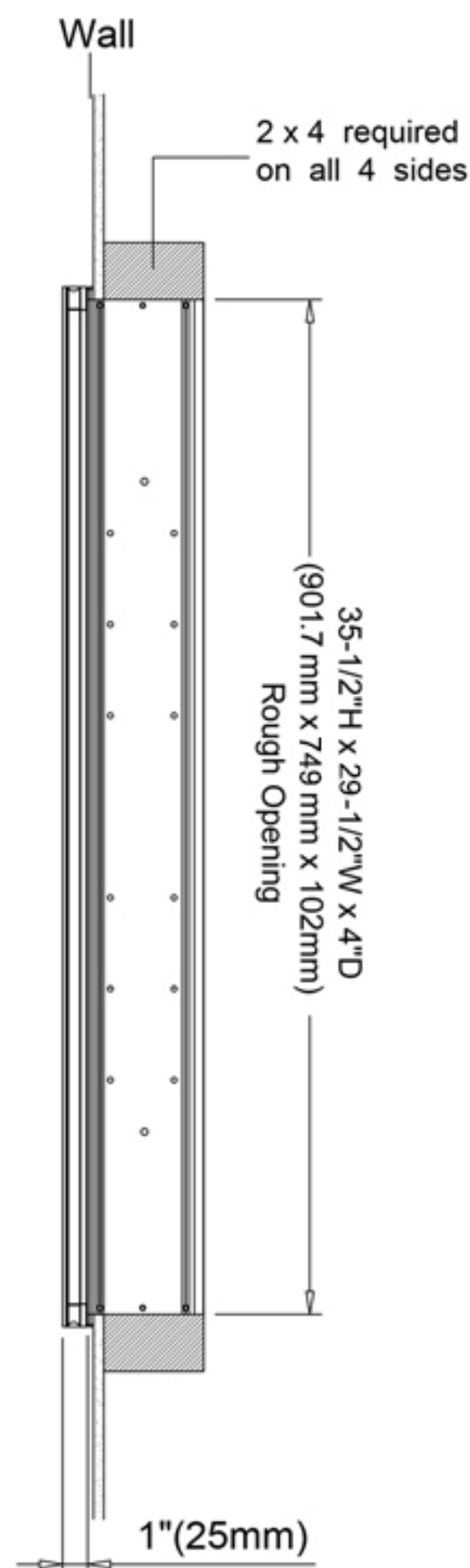
Recessed Mount
