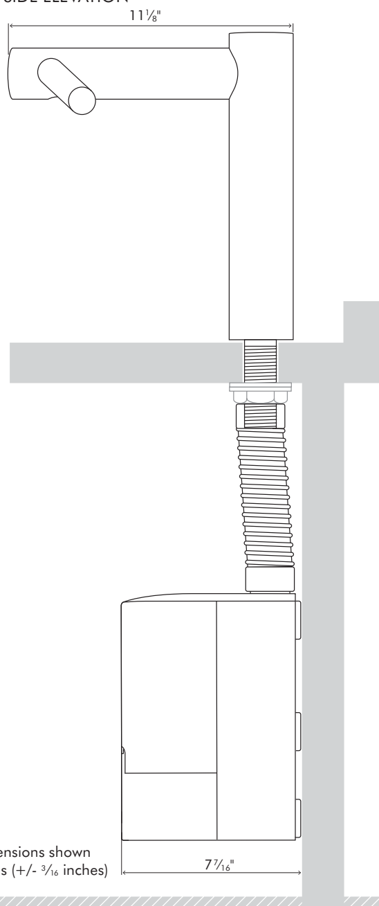
SIDE ELEVATION
