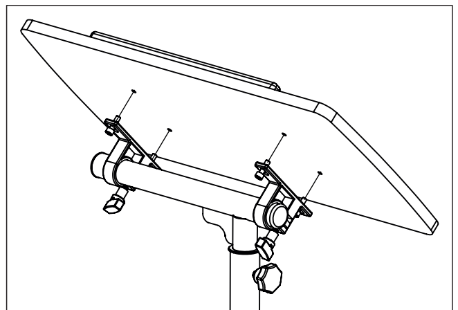
Attaching the wooden top to the metal frame
