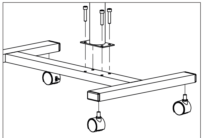
Attaching the wheels and vertical section to the I frame
