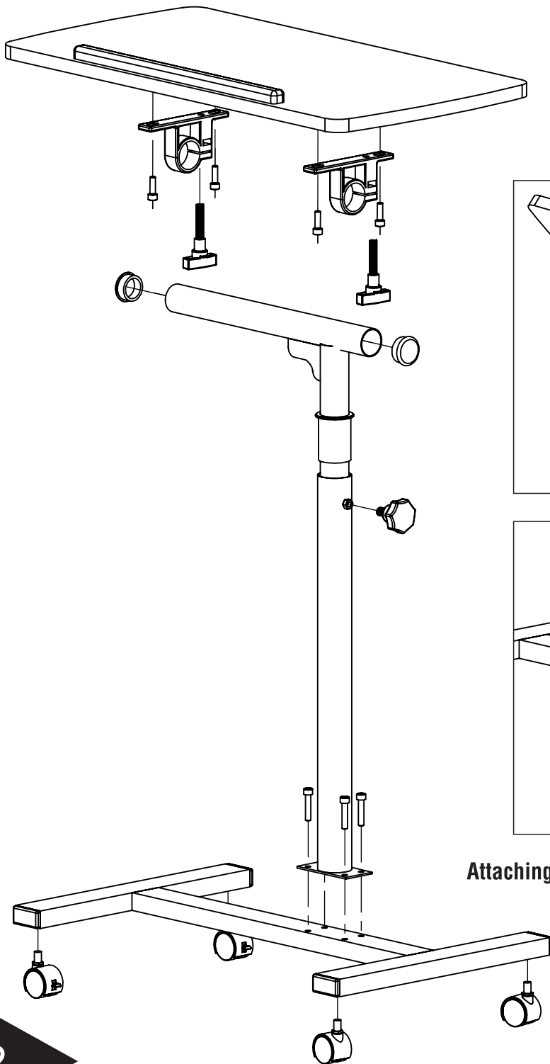
Attaching the wooden top to the metal frame
