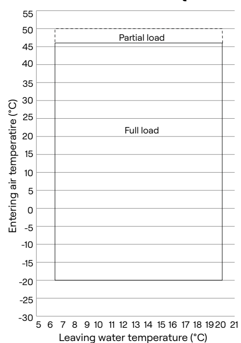
Operating map - cooling mode Standard unit 61AQ
