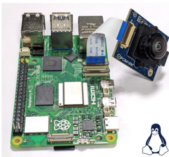
Figure 3. Typical setup when using VD56G3 S-Board on an embedded processing platform
