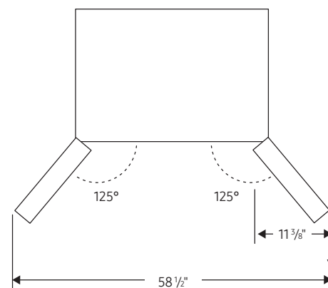
TOP OF REFRIGERATOR WITH DOORS OPEN 125^\circ
