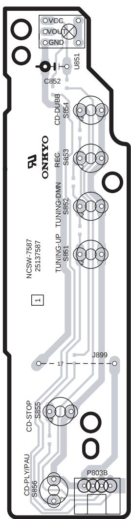
Component side
