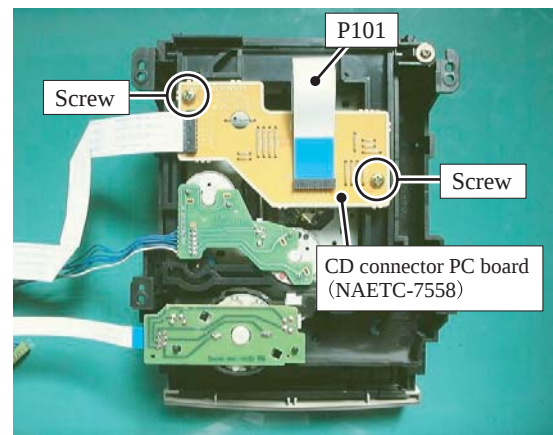
--Bottom view of CD mechanism--
