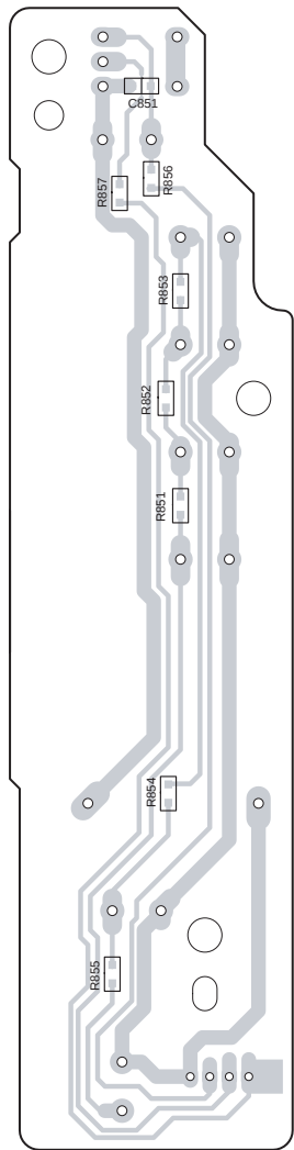
Soldering side
