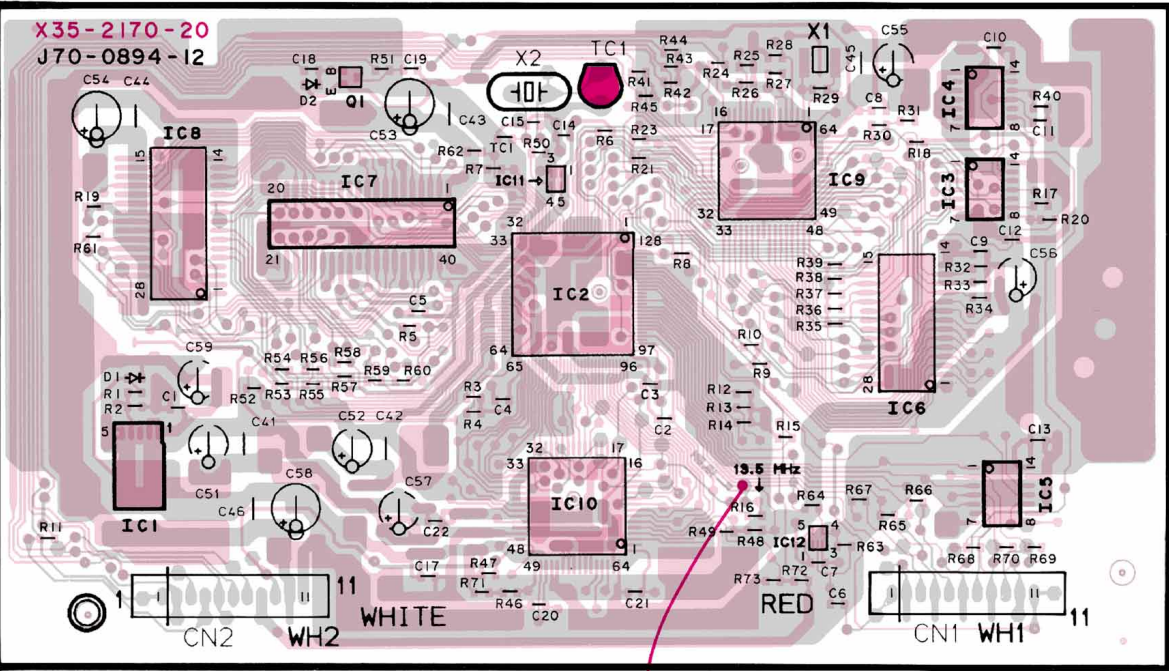
Video unit (X35-2170-20)
