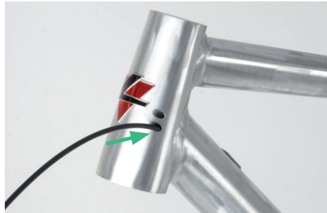
1. Insert the shifting cable housing into the left-hand bottom hole underneath the headset.
