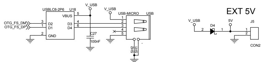
Figure 3. STEVAL-STWINKT1B schematic (1 of 7)
