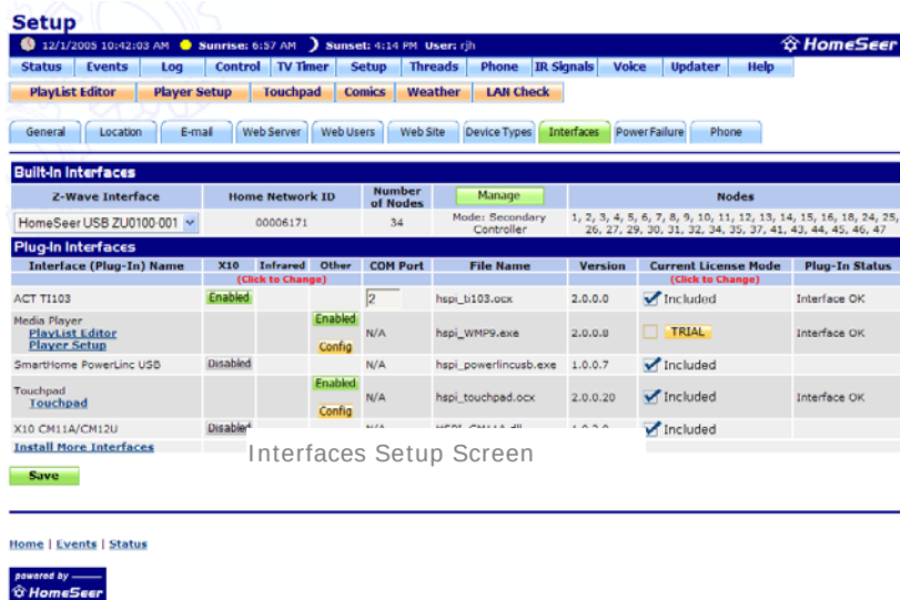
Figure 4: Interface Setup
