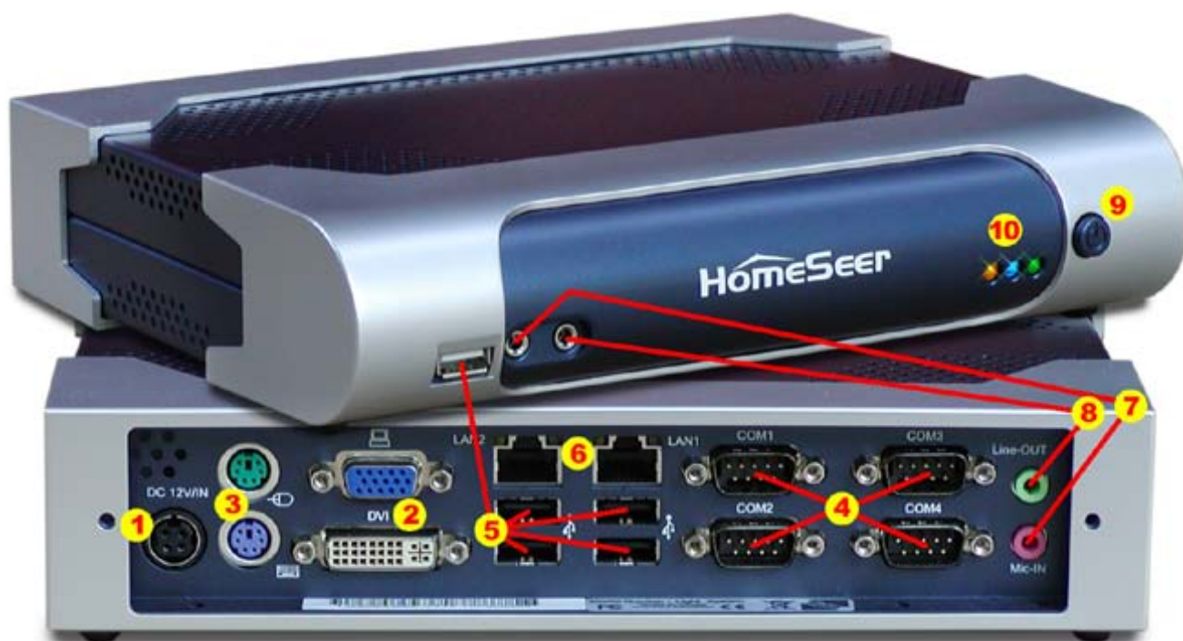
Figure 1: Front / Rear Panel of HomeTroller
