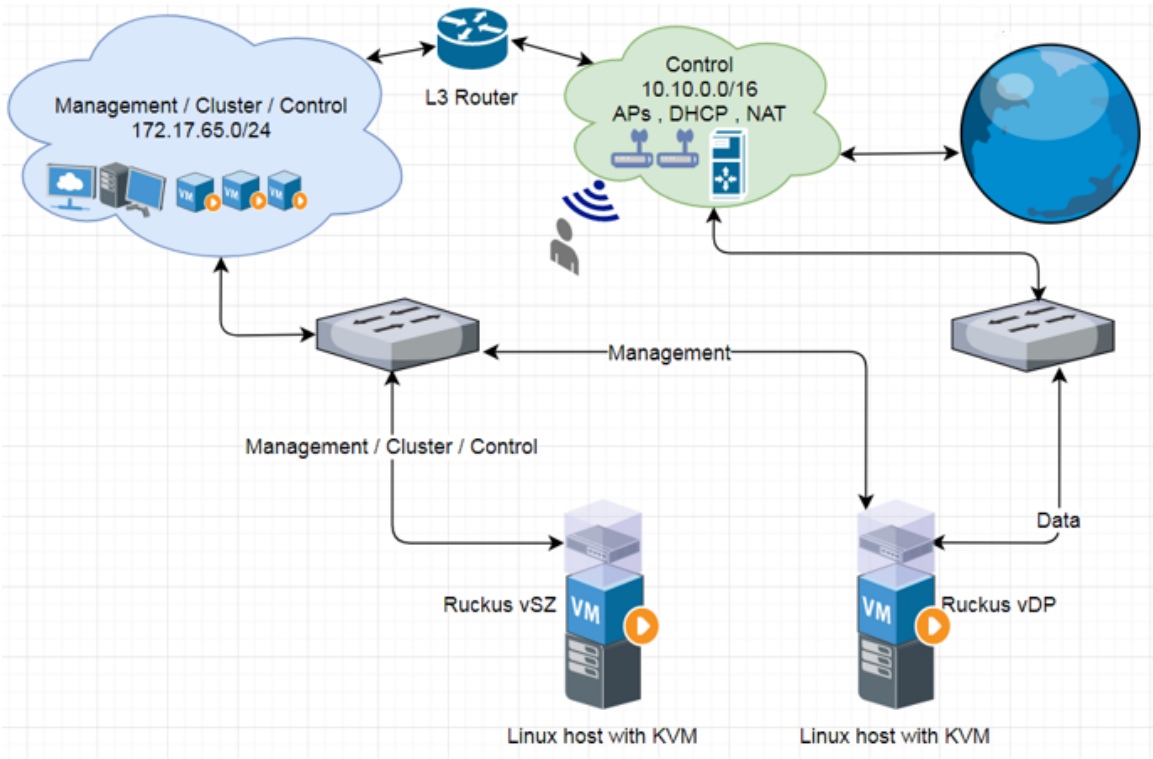
FIGURE 40 Two different domain IP addresses setup
