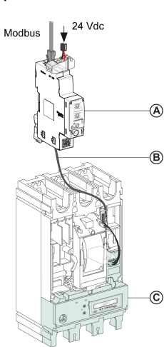
Example 1: Connection of the IFM interface to the MicroLogic 5, 6, or 7 trip unit
