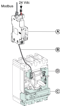
Example 3: Connection of the IFM interface to the BSCM module and the MicroLogic 5, 6, or 7 trip unit
