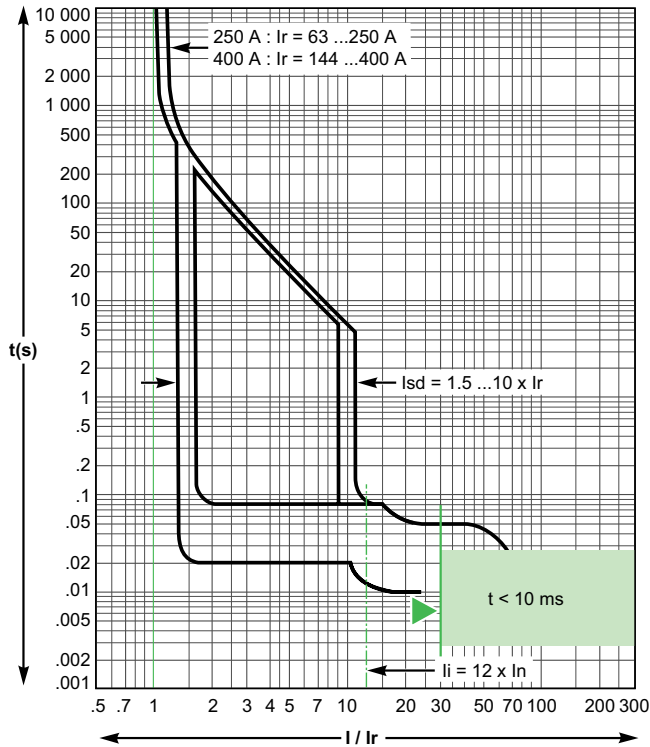
MicroLogic 2.3 and 4.3 - 250–400 A
