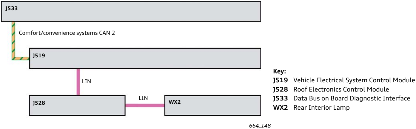
Schematic diagram – Networking of both overhead modules
