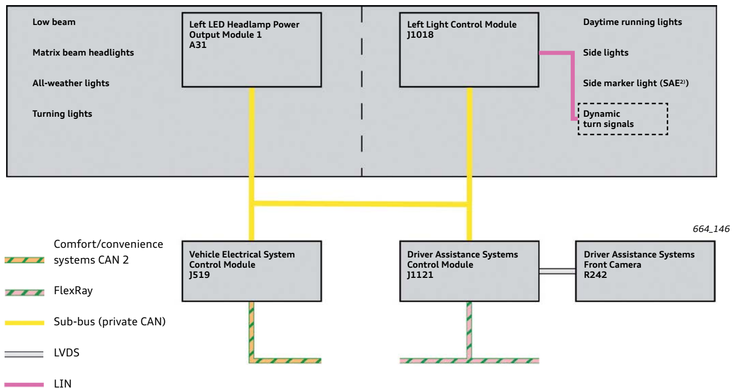
Schematic diagram of the left headlight
