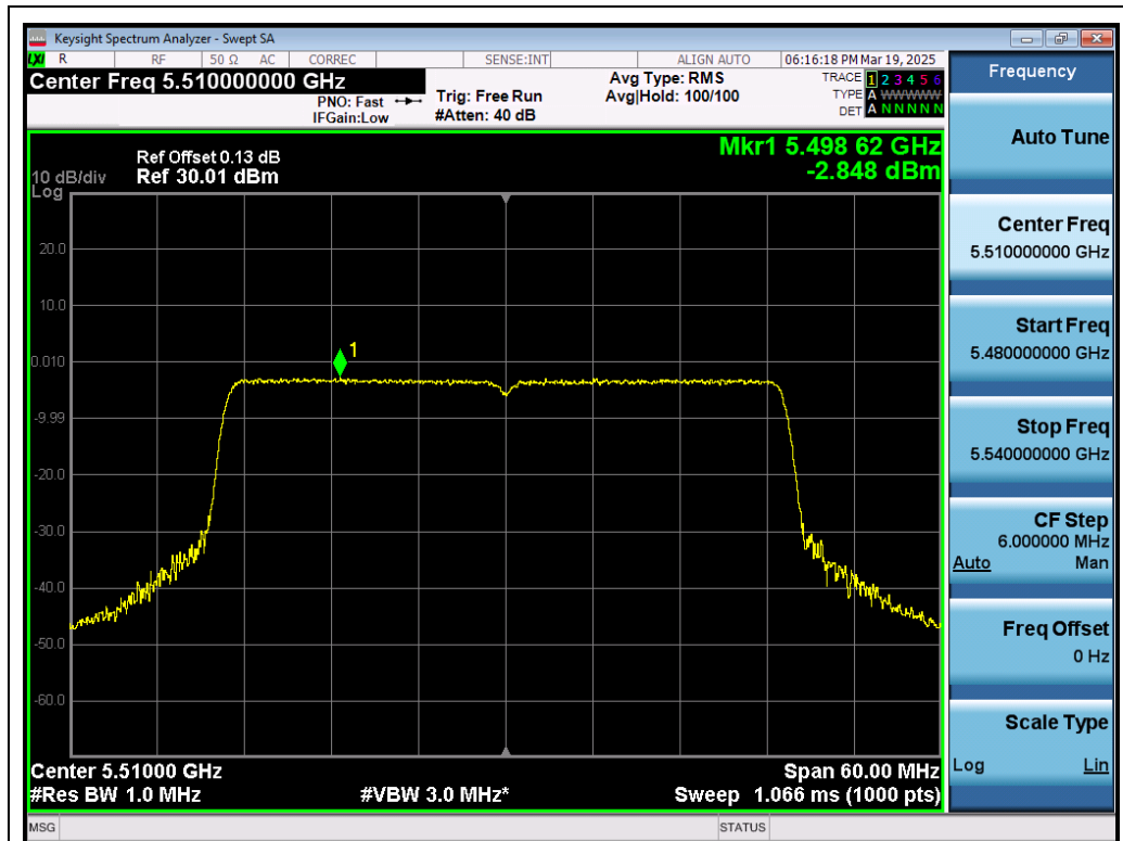
Test_Graph_802.11ax40_ANT1_5510_MCS0_PSD
