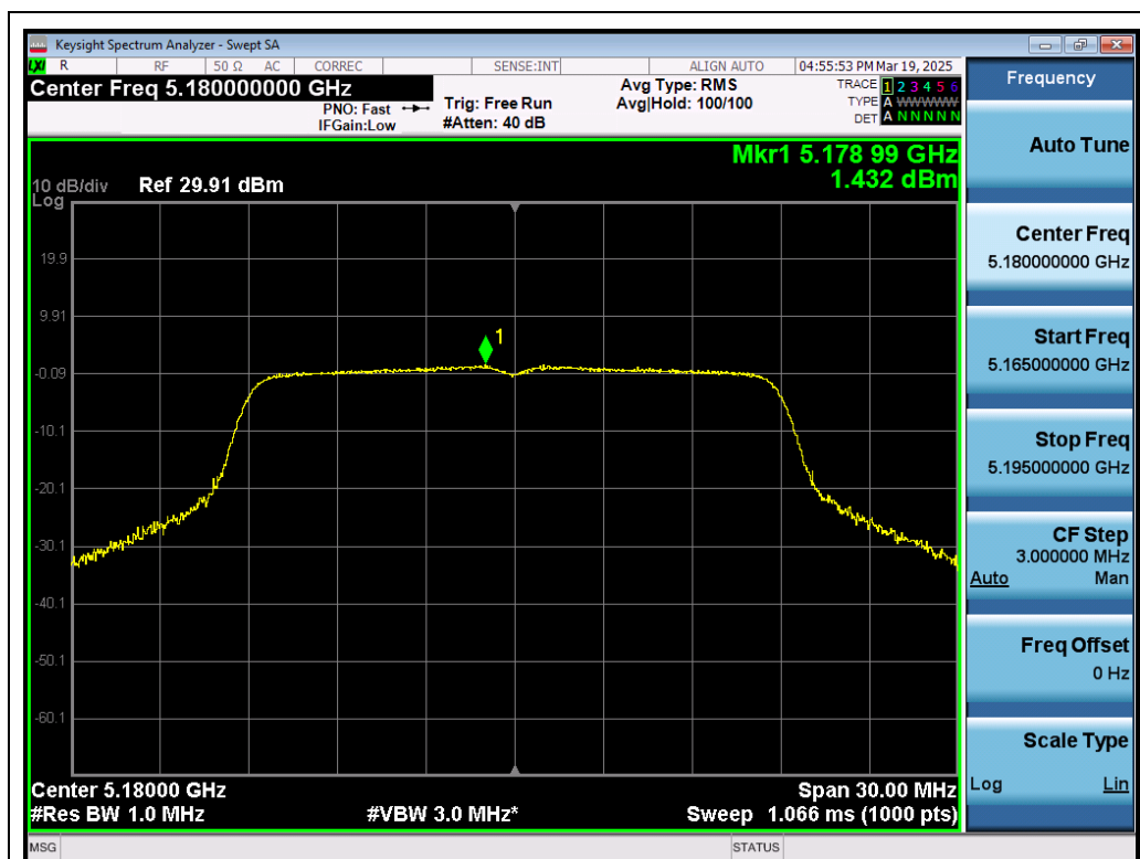
Test_Graph_802.11ac20_ANT1_5180_MCS0_PSD
