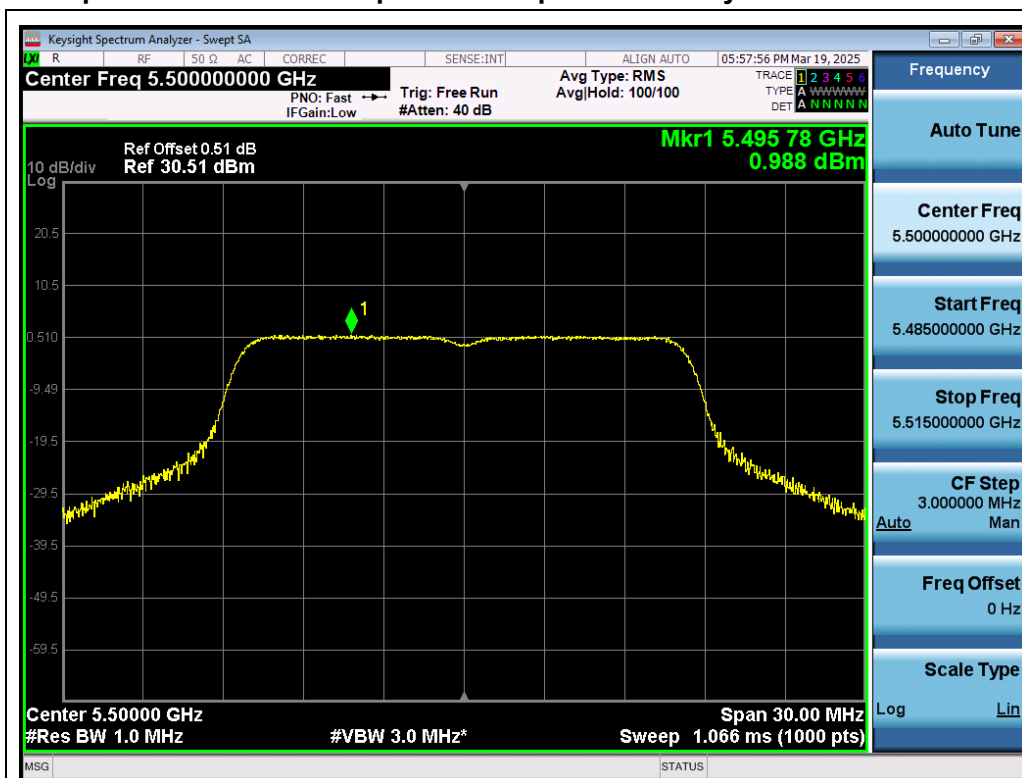
Test_Graph_802.11a_ANT1_5500_6Mbps_PSD
