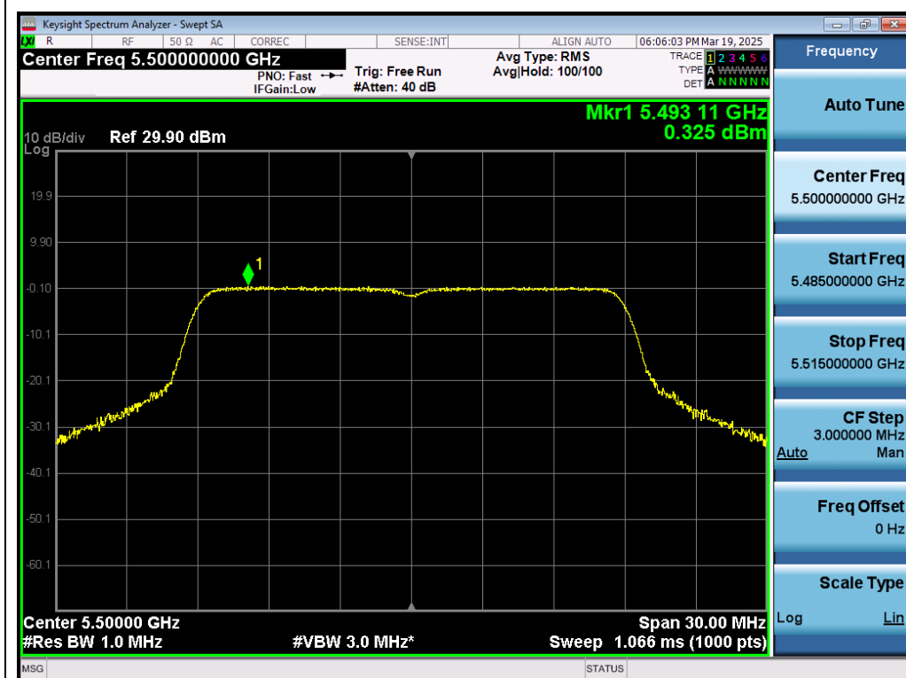
Test_Graph_802.11ac20_ANT1_5500_MCS0_PSD
