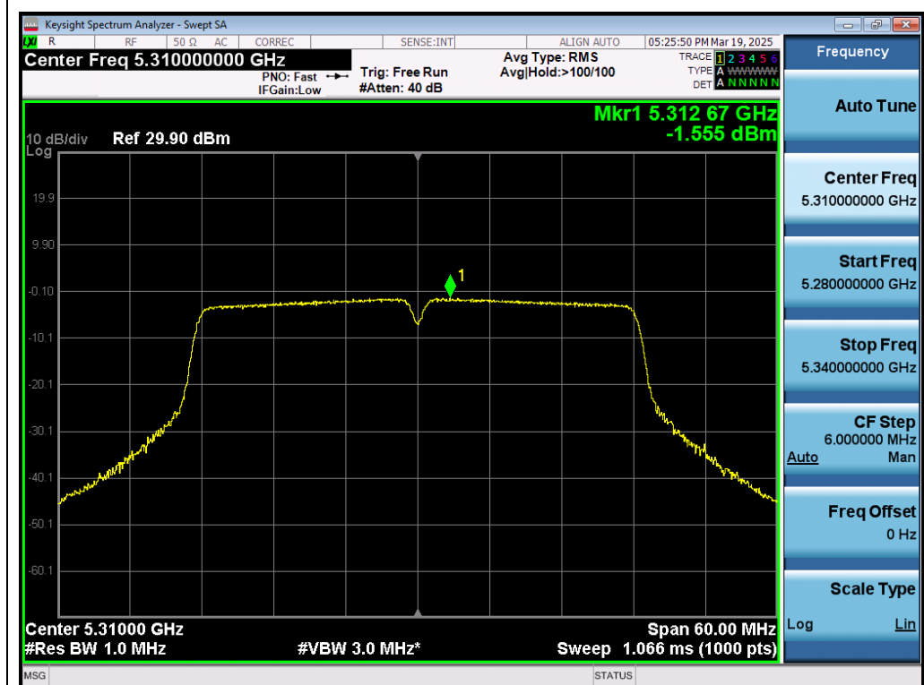
Test_Graph_802.11n40_ANT1_5310_MCS0_PSD
