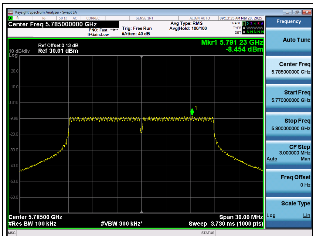
Test_Graph_802.11n20_ANT1_5785_MCS0_PSD
