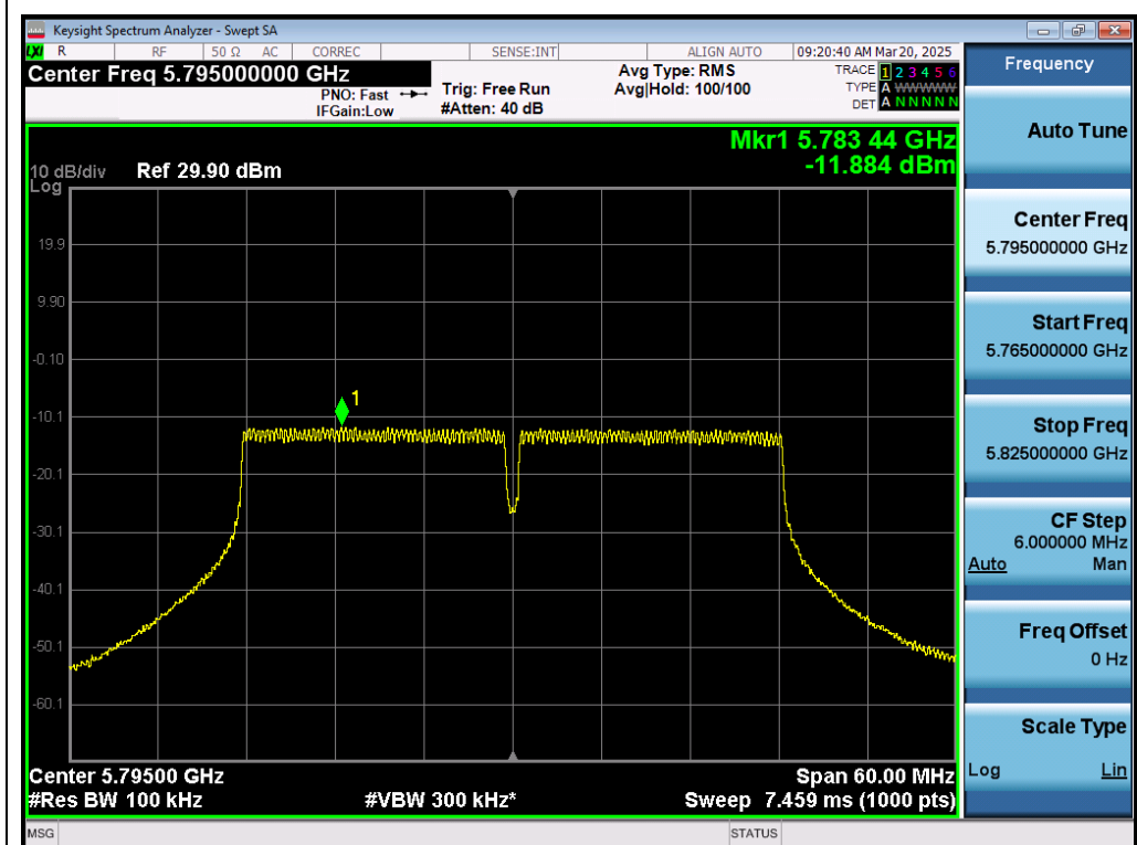
Test_Graph_802.11n40_ANT1_5795_MCS0_PSD
