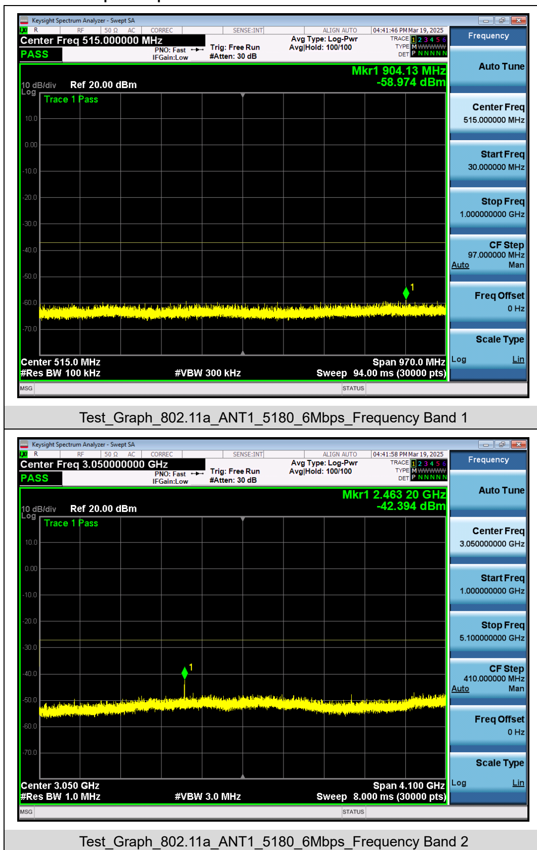
Test Graphs of Spurious Emissions outside of the 5.15-5.25 GHz band
