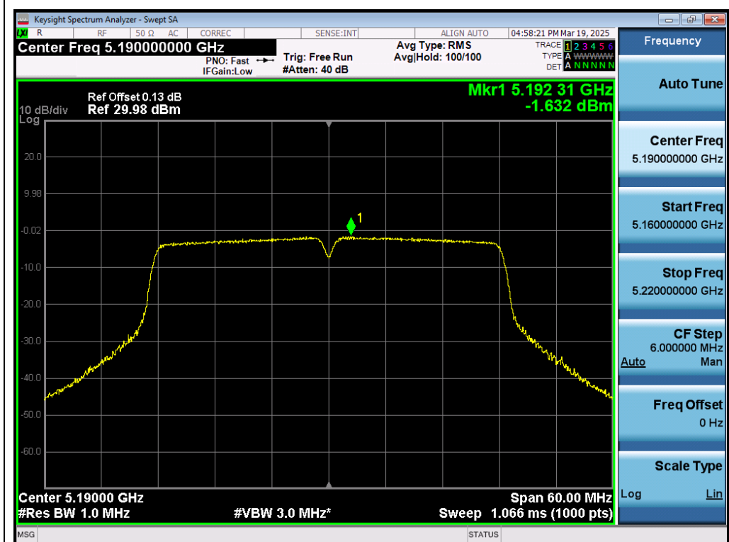
Test_Graph_802.11ac40_ANT1_5190_MCS0_PSD
