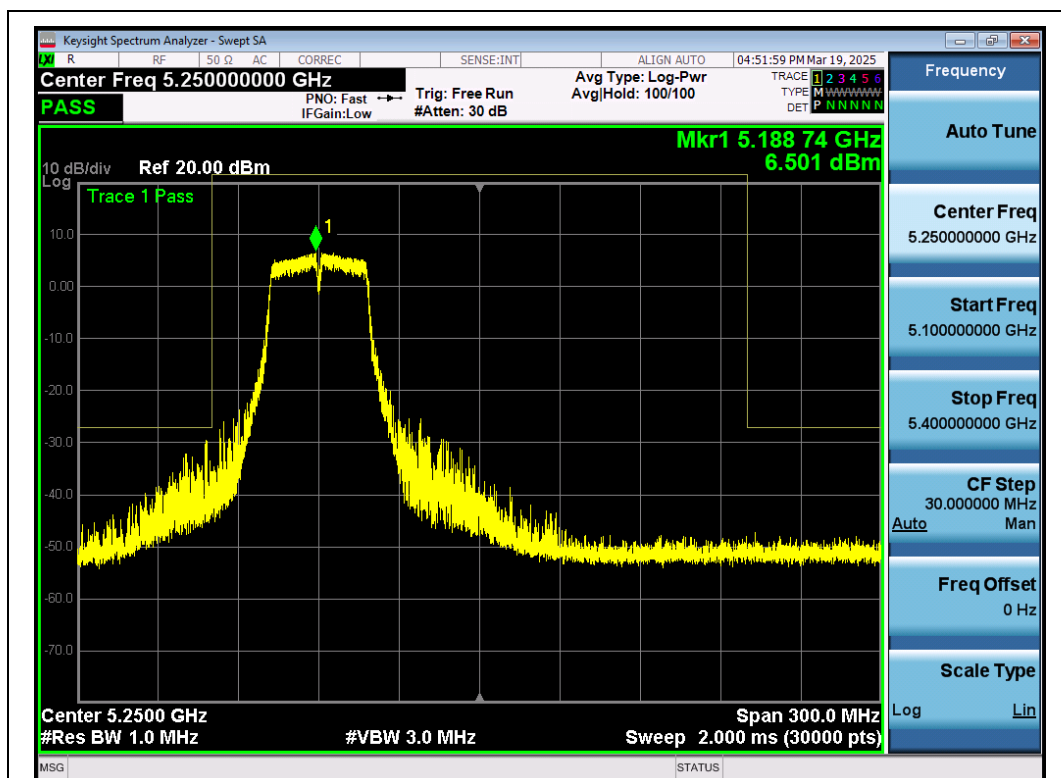
Test_Graph_802.11n40_ANT1_5190_MCS0_Frequency Band 3
