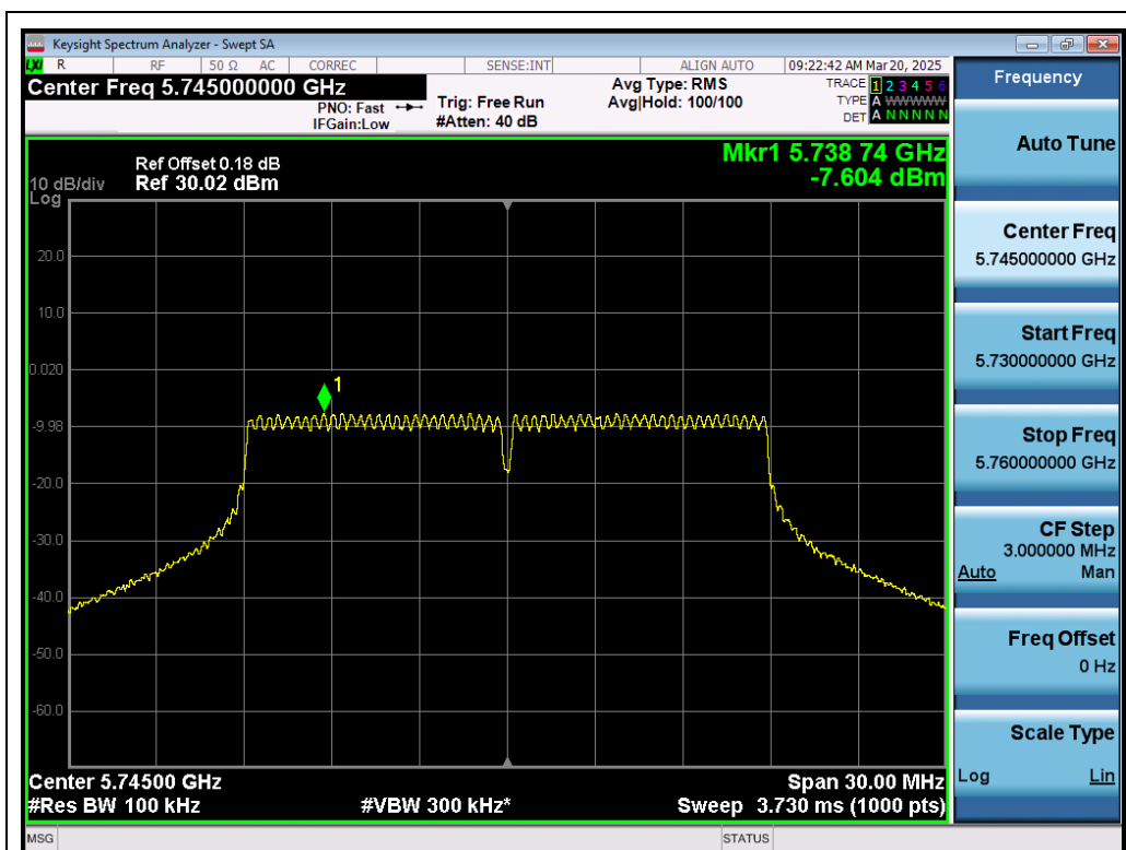
Test_Graph_802.11ac20_ANT1_5745_MCS0_PSD
