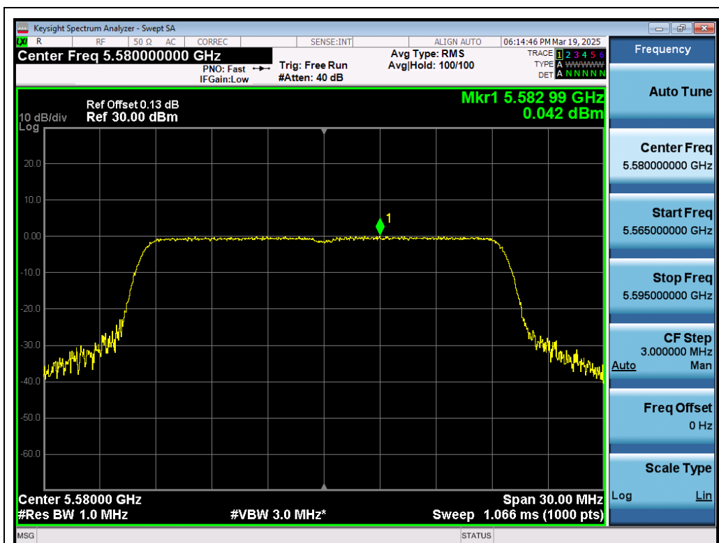
Test_Graph_802.11ax20_ANT1_5580_MCS0_PSD
