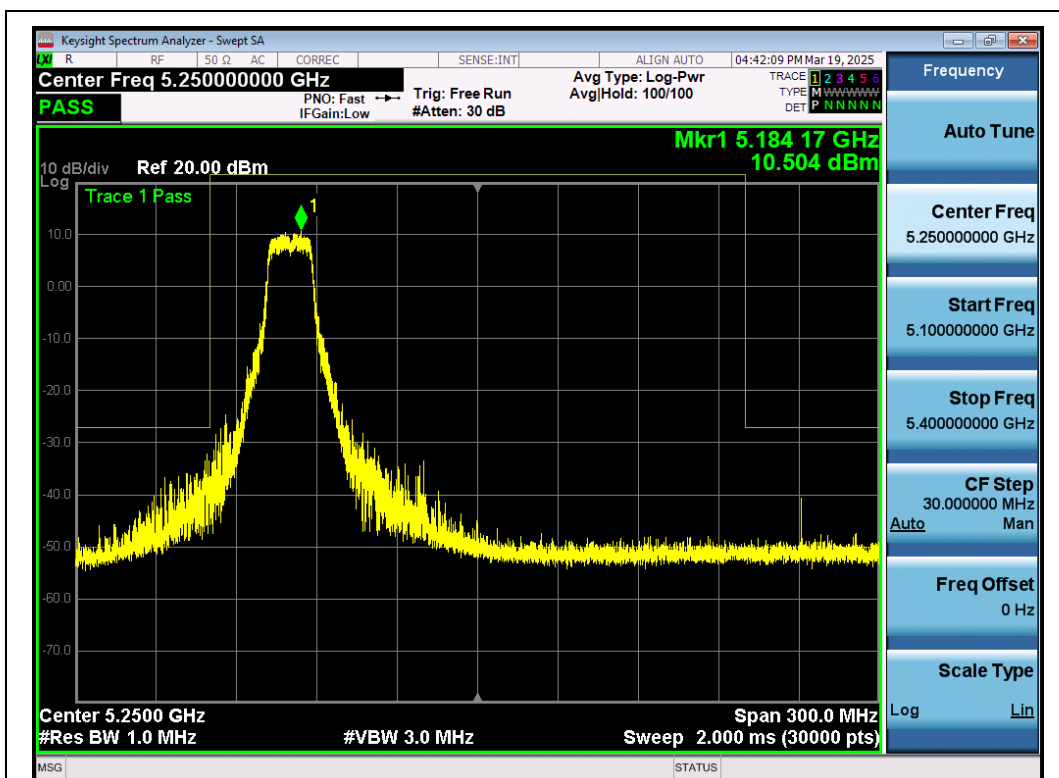
Test_Graph_802.11a_ANT1_5180_6Mbps_Frequency Band 3
