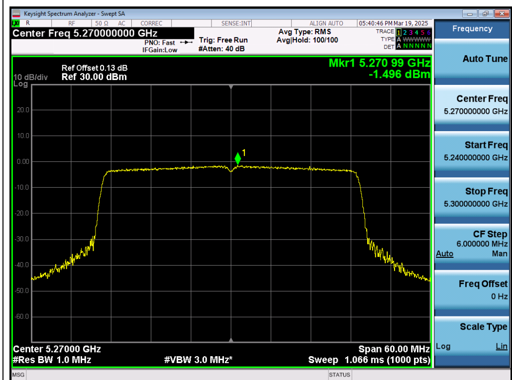
Test_Graph_802.11ax40_ANT1_5270_MCS0_PSD
