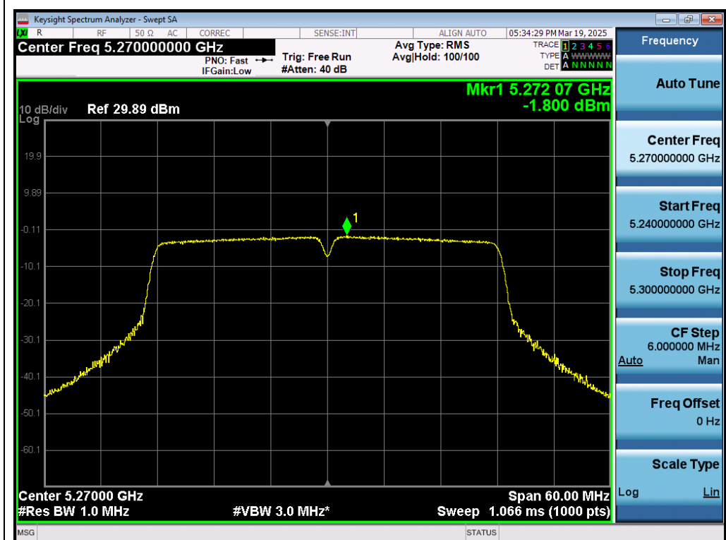
Test_Graph_802.11ac40_ANT1_5270_MCS0_PSD
