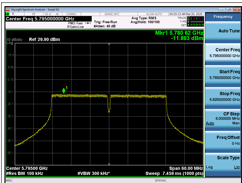
Test_Graph_802.11ac40_ANT1_5795_MCS0_PSD
