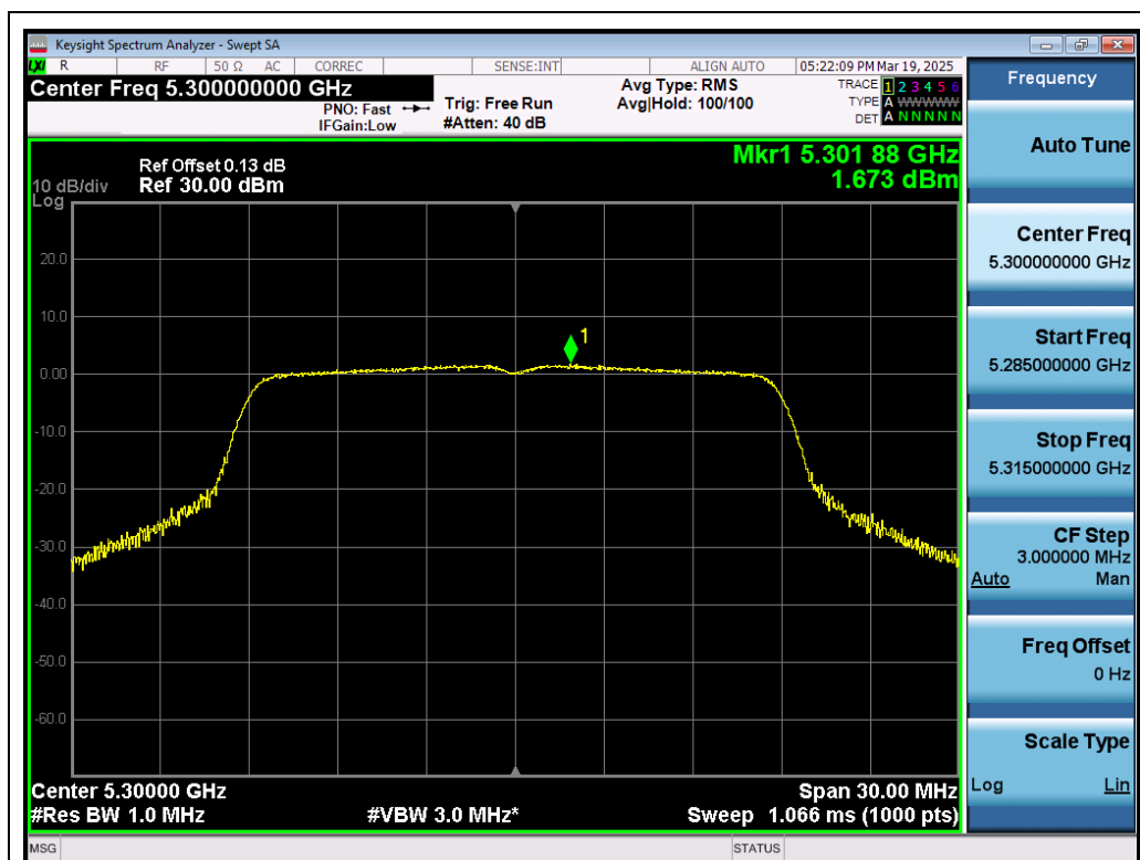
Test_Graph_802.11n20_ANT1_5300_MCS0_PSD
