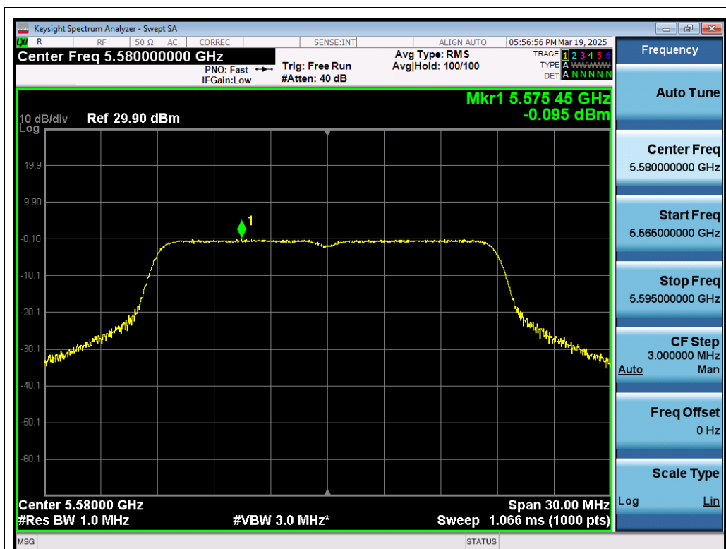
Test_Graph_802.11n20_ANT1_5580_MCS0_PSD
