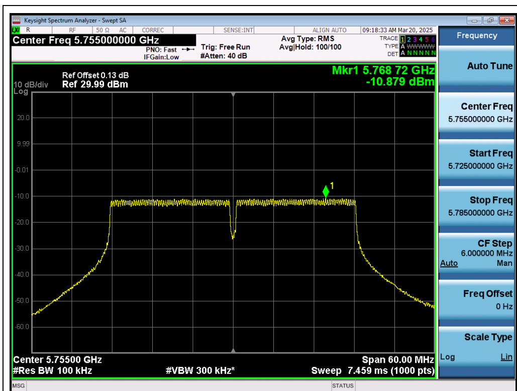
Test_Graph_802.11n40_ANT1_5755_MCS0_PSD
