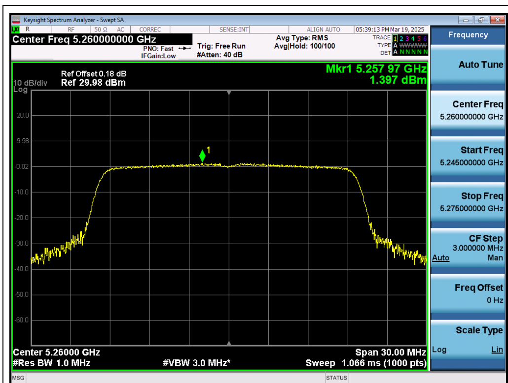
Test_Graph_802.11ax20_ANT1_5260_MCS0_PSD
