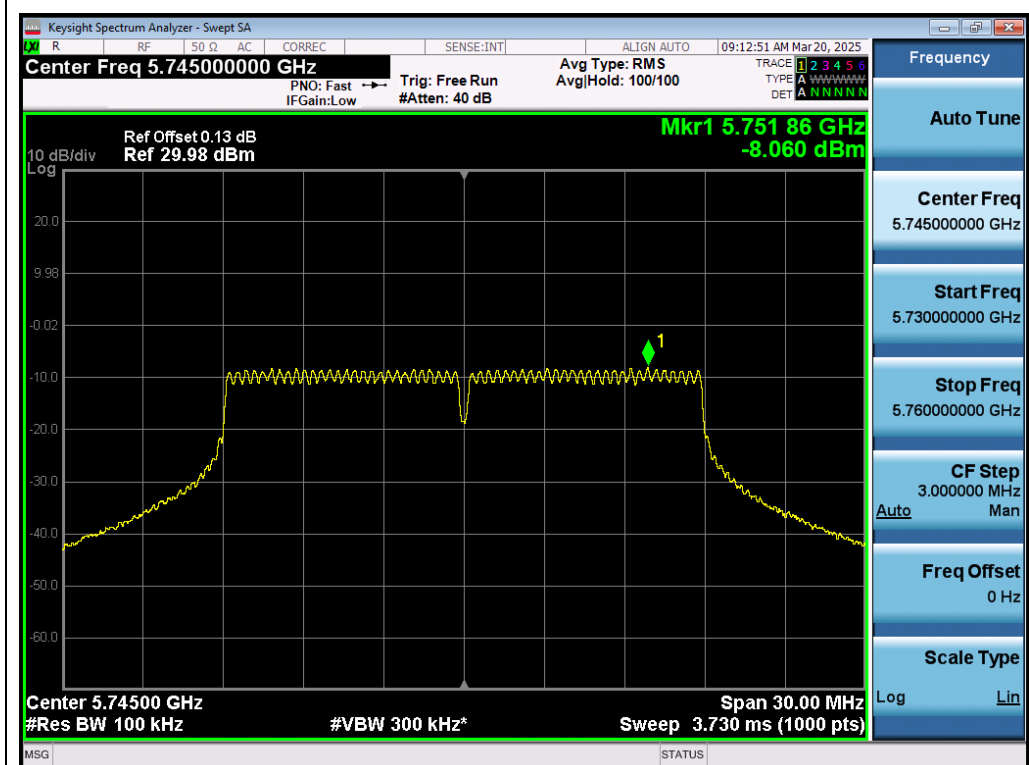
Test_Graph_802.11n20_ANT1_5745_MCS0_PSD
