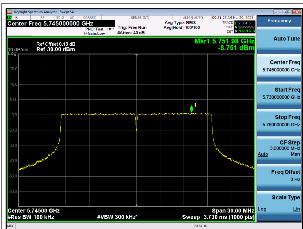
Test_Graph_802.11ax20_ANT1_5745_MCS0_PSD
