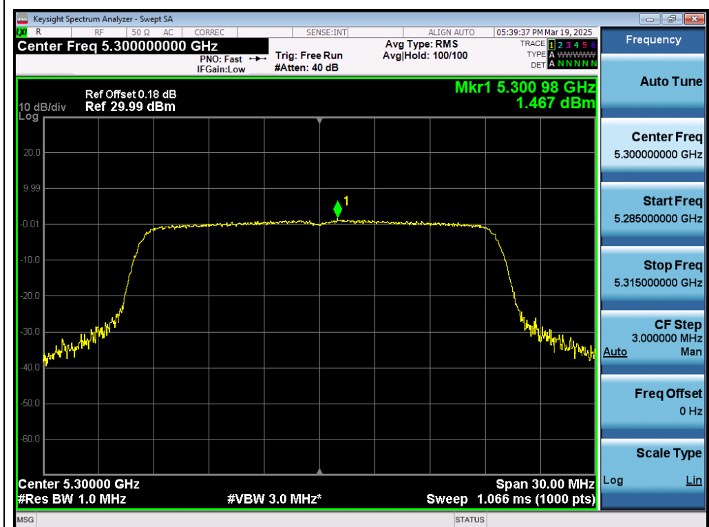
Test_Graph_802.11ax20_ANT1_5300_MCS0_PSD
