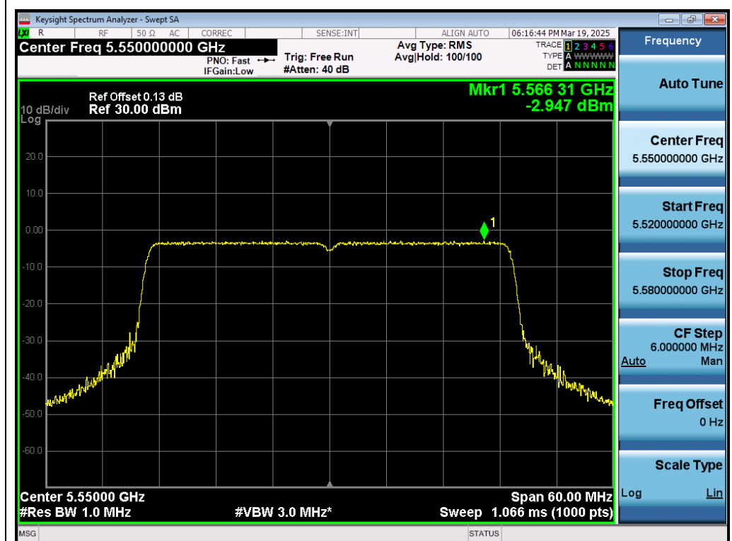
Test_Graph_802.11ax40_ANT1_5550_MCS0_PSD
