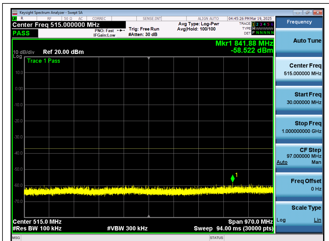
Test_Graph_802.11a_ANT1_5240_6Mbps_Frequency Band 1
