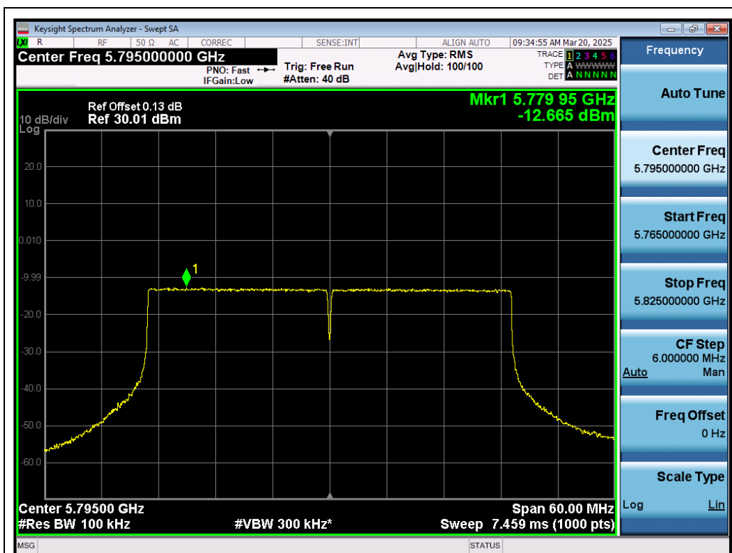
Test_Graph_802.11ax40_ANT1_5795_MCS0_PSD
