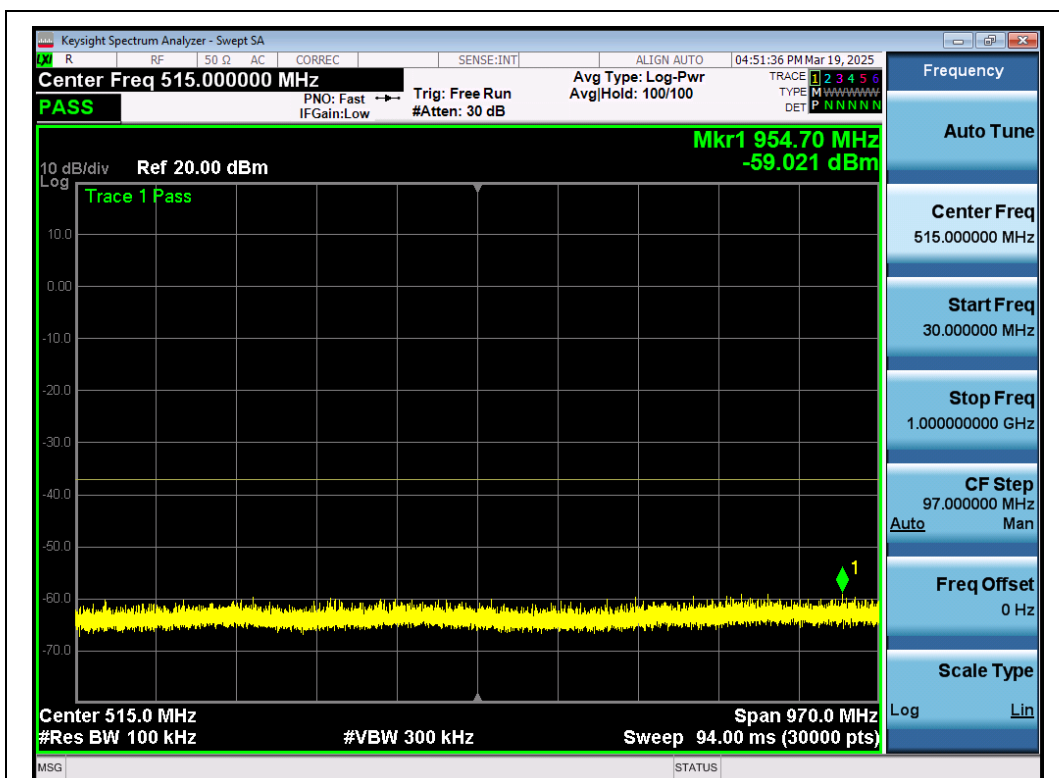
Test_Graph_802.11n40_ANT1_5190_MCS0_Frequency Band 1
