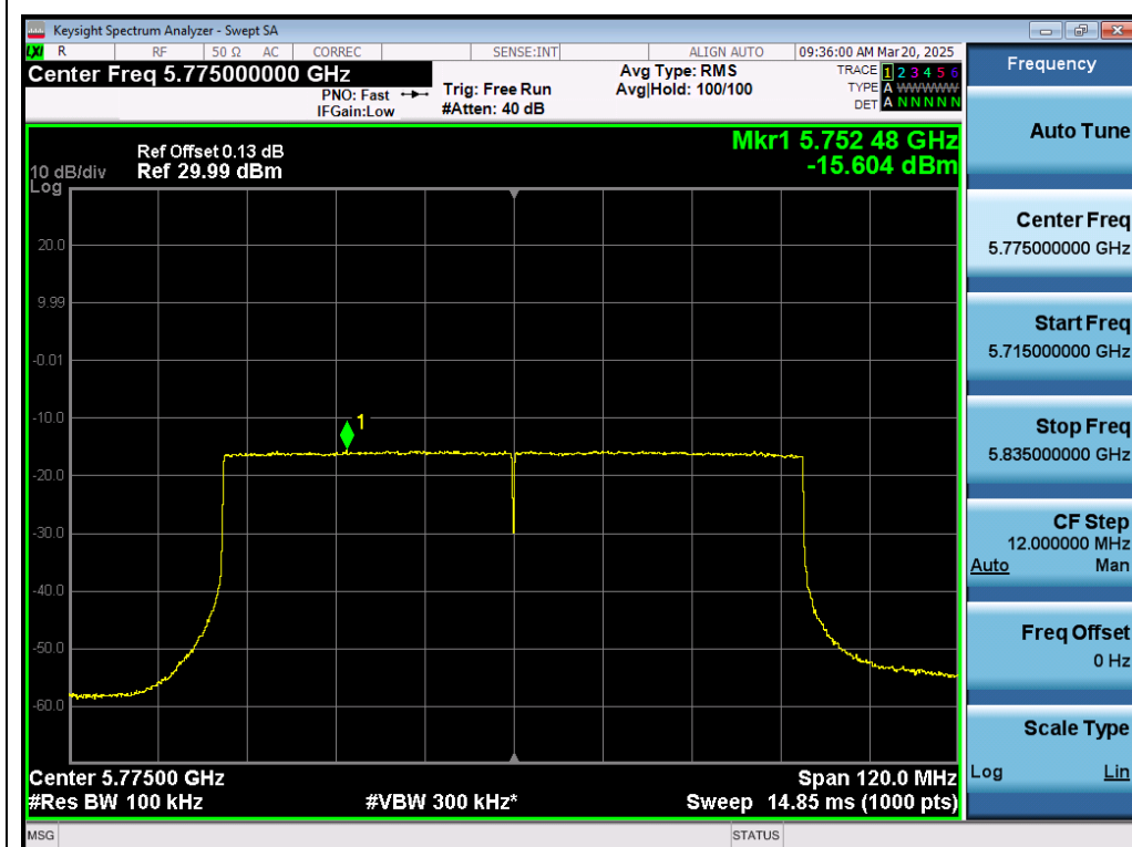
Test_Graph_802.11ax80_ANT1_5775_MCS0_PSD
