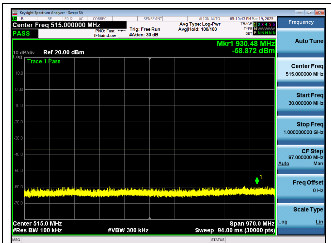
Test_Graph_802.11ax80_ANT1_5210_MCS0_Frequency Band 1
