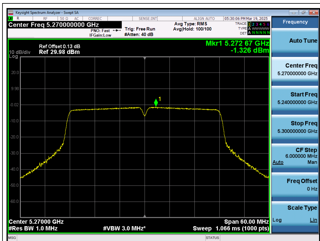
Test_Graph_802.11n40_ANT1_5270_MCS0_PSD
