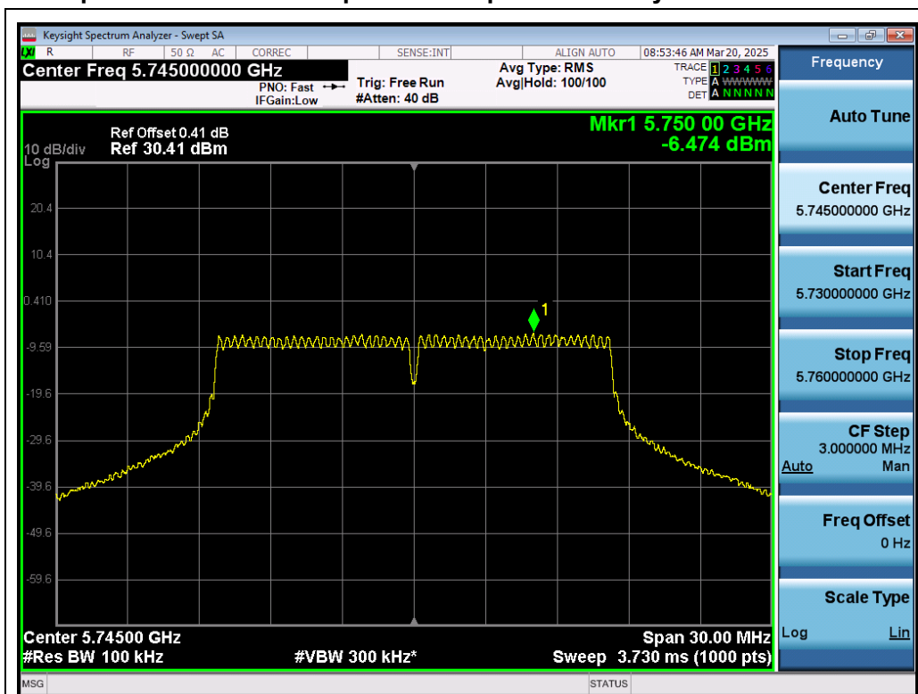
Test_Graph_802.11a_ANT1_5745_6Mbps_PSD
