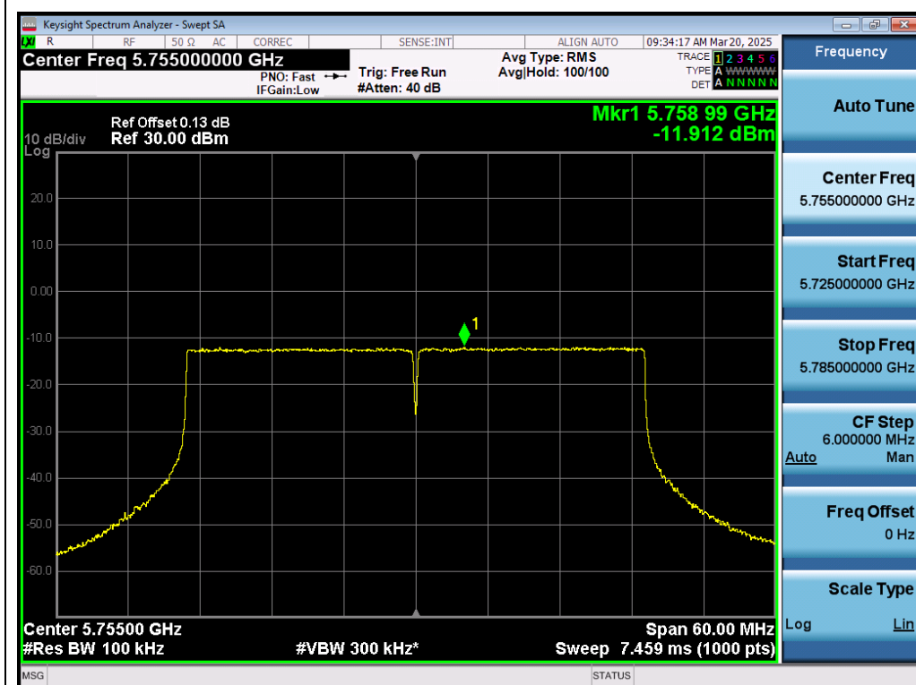
Test_Graph_802.11ax40_ANT1_5755_MCS0_PSD
