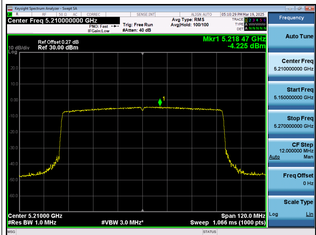
Test_Graph_802.11ax80_ANT1_5210_MCS0_PSD
