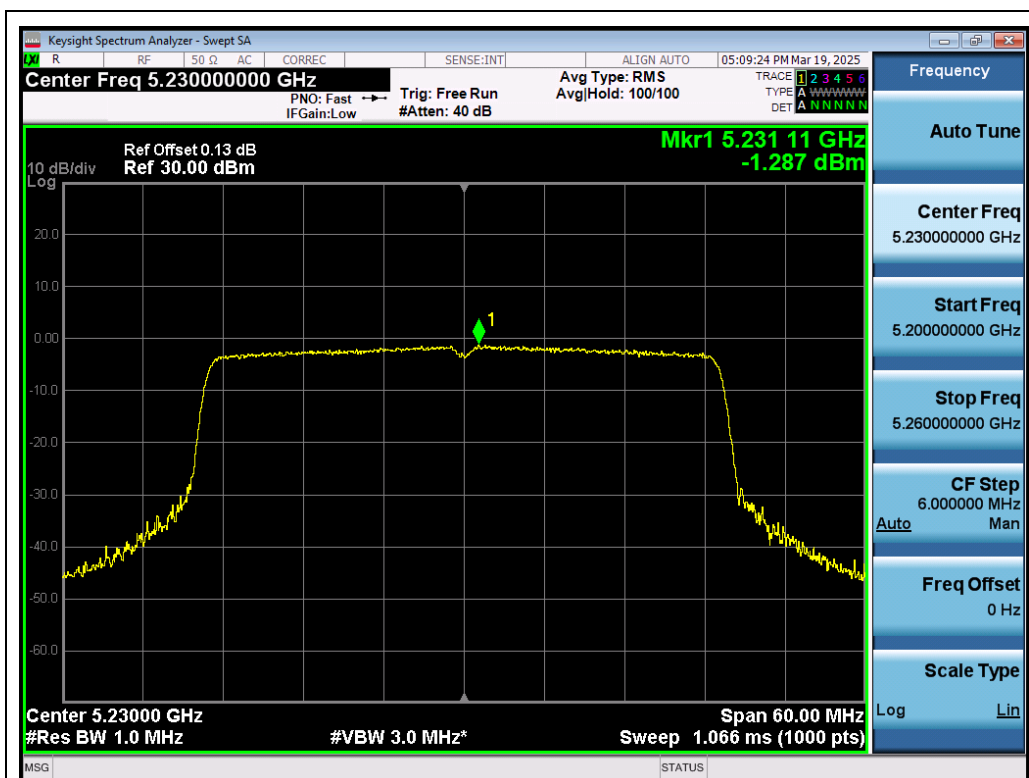
Test_Graph_802.11ax40_ANT1_5230_MCS0_PSD
