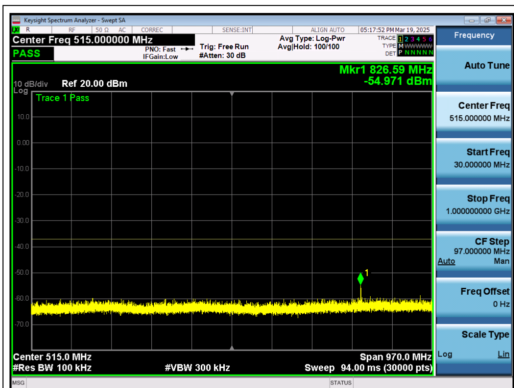
Test_Graph_802.11a_ANT1_5320_6Mbps_Frequency Band 1
