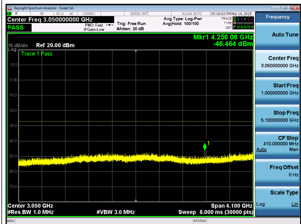
Test_Graph_802.11a_ANT1_5320_6Mbps_Frequency Band 2
