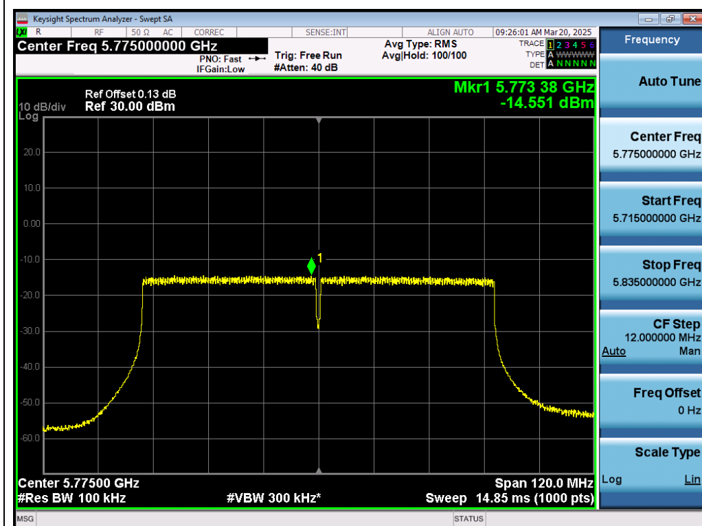
Test_Graph_802.11ac80_ANT1_5775_MCS0_PSD
