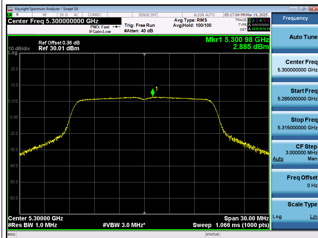
Test_Graph_802.11a_ANT1_5300_6Mbps_PSD
