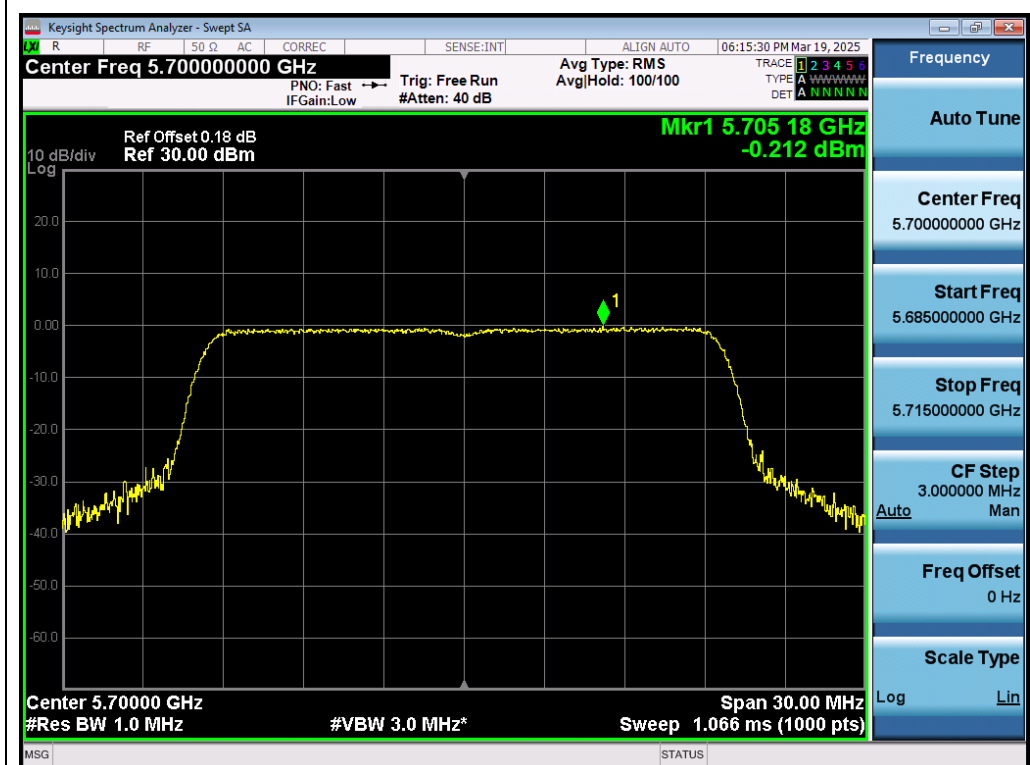
Test_Graph_802.11ax20_ANT1_5700_MCS0_PSD
