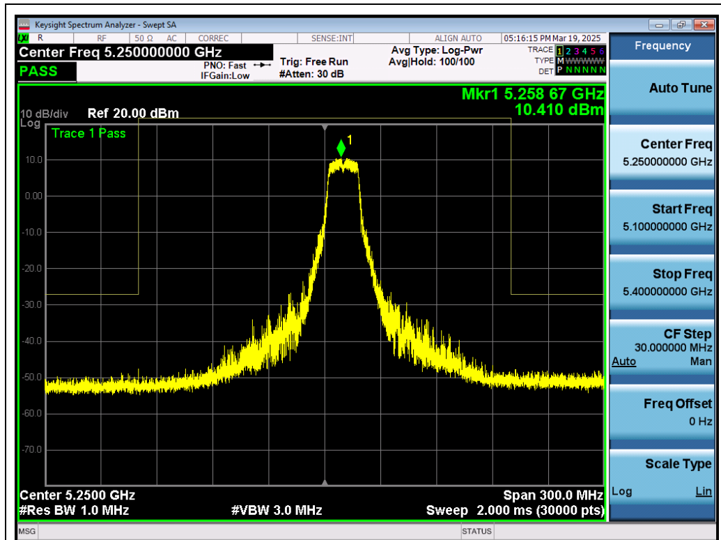
Test_Graph_802.11a_ANT1_5260_6Mbps_Frequency Band 3
