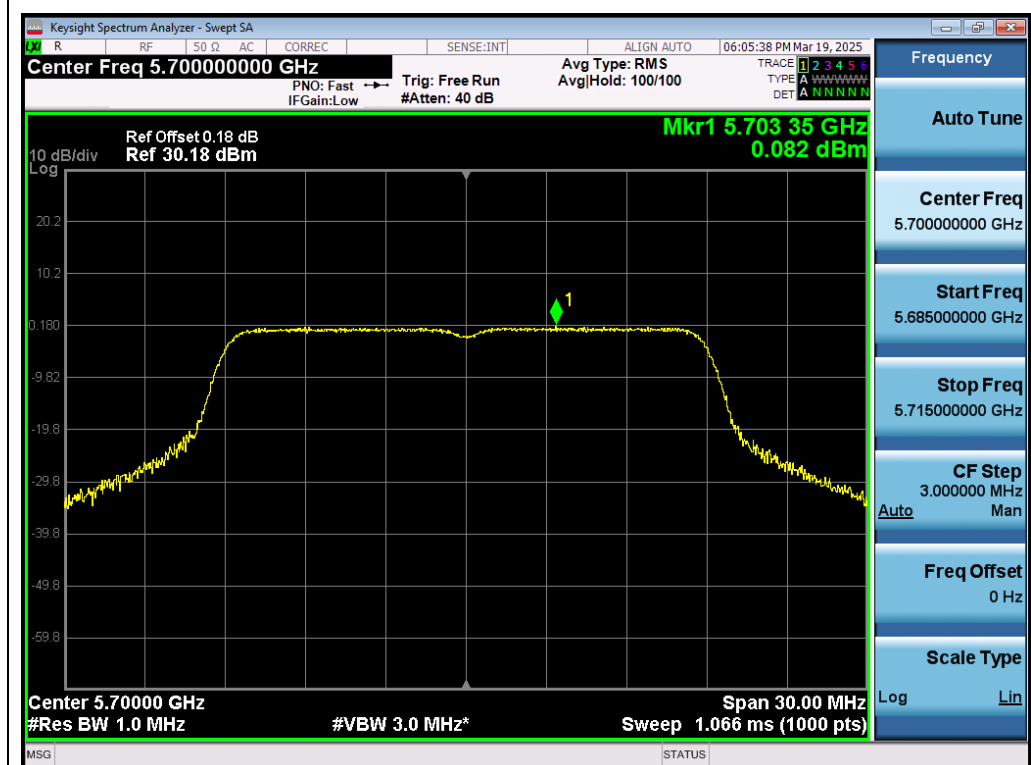
Test_Graph_802.11ac20_ANT1_5700_MCS0_PSD
