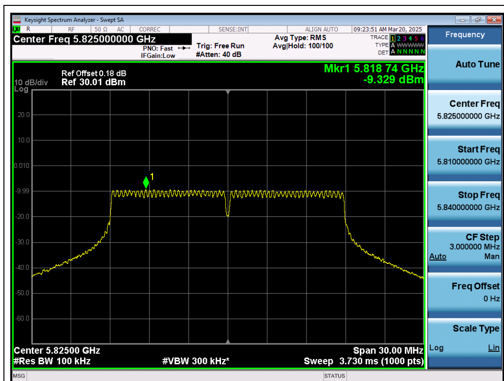
Test_Graph_802.11ac20_ANT1_5825_MCS0_PSD
