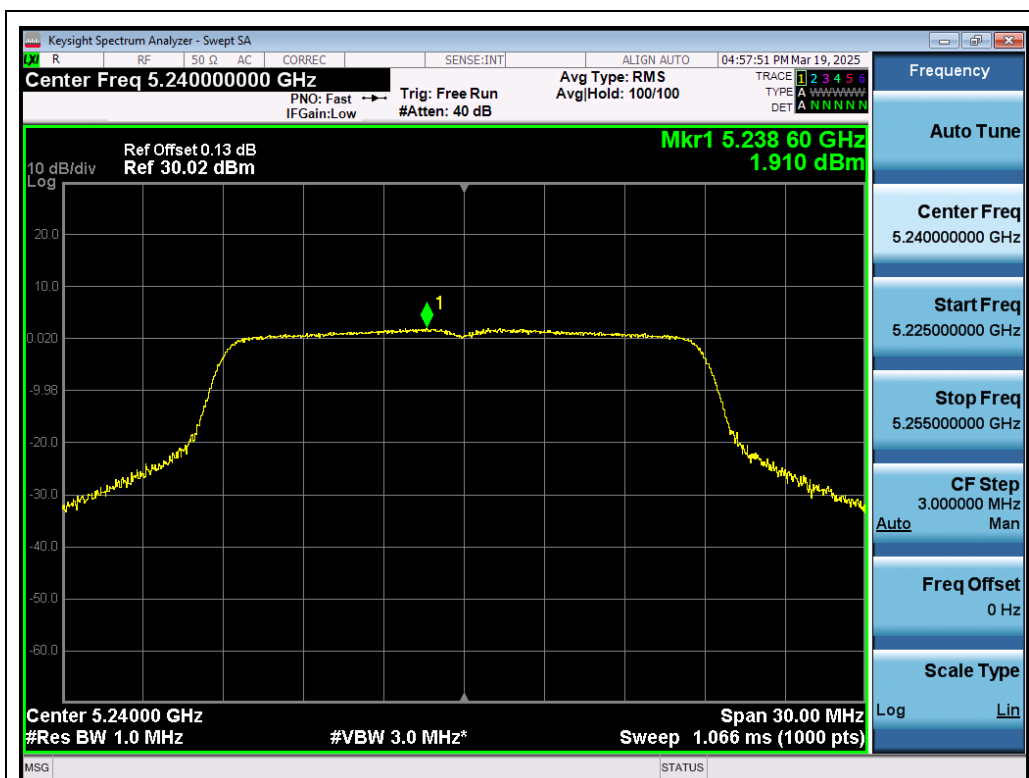
Test_Graph_802.11ac20_ANT1_5240_MCS0_PSD
