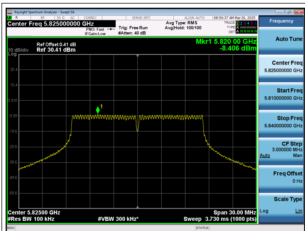
Test_Graph_802.11a_ANT1_5825_6Mbps_PSD
