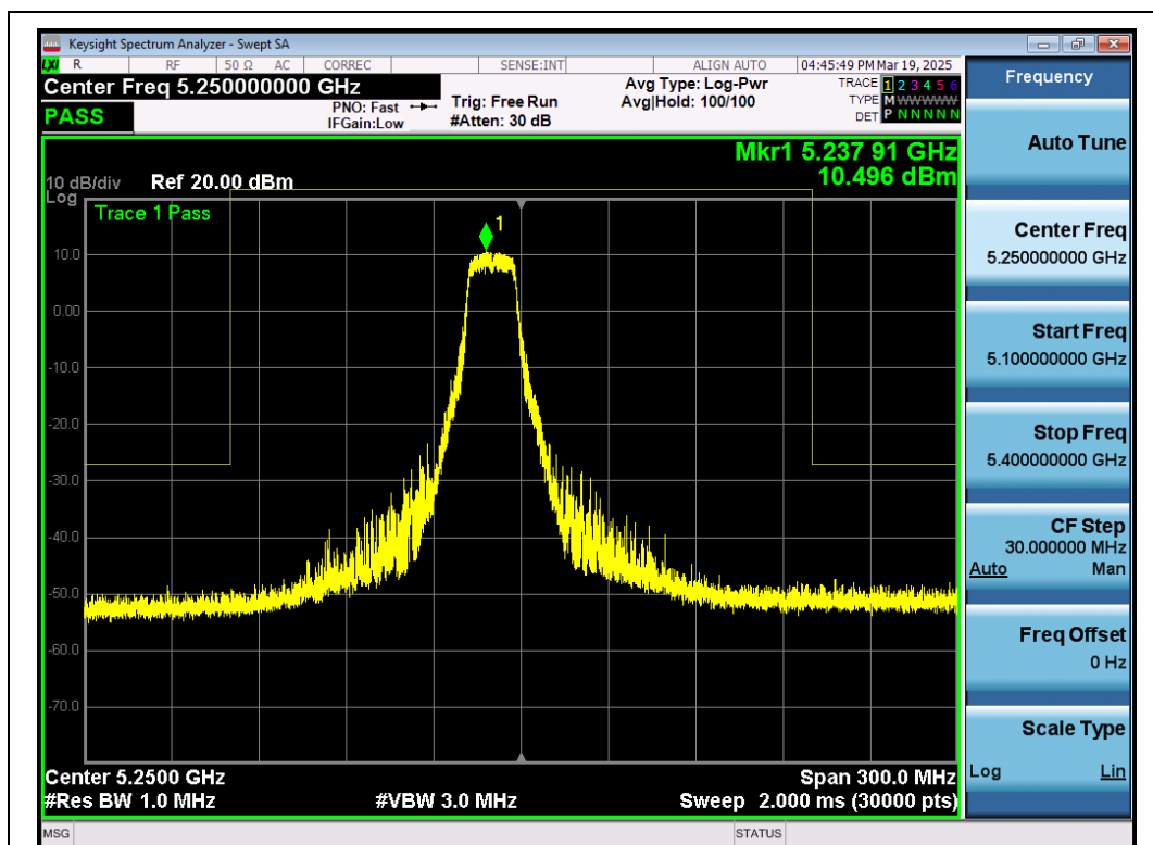
Test_Graph_802.11a_ANT1_5240_6Mbps_Frequency Band 3
