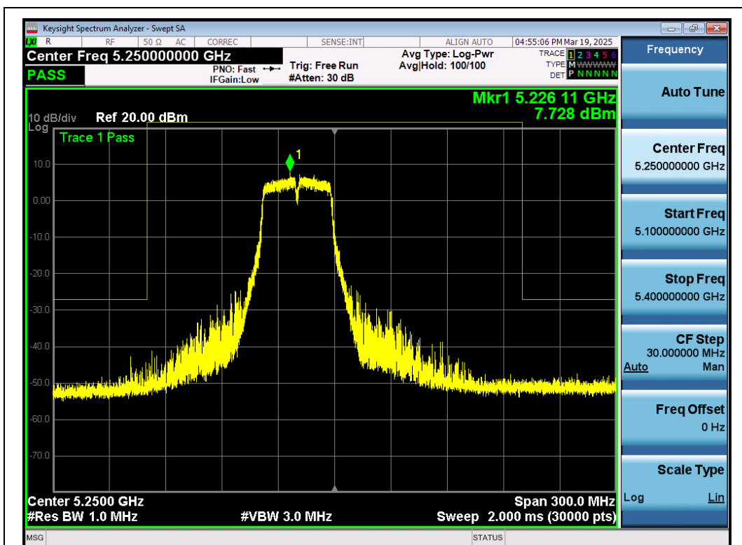
Test_Graph_802.11n40_ANT1_5230_MCS0_Frequency Band 3
