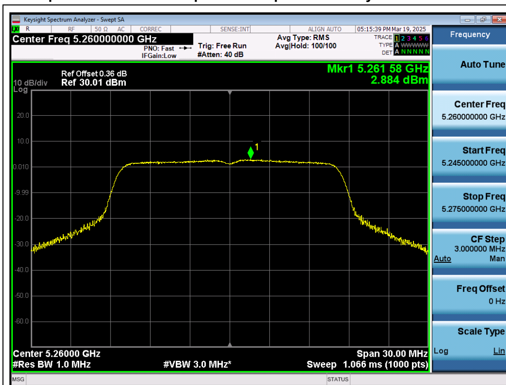
Test_Graph_802.11a_ANT1_5260_6Mbps_PSD
