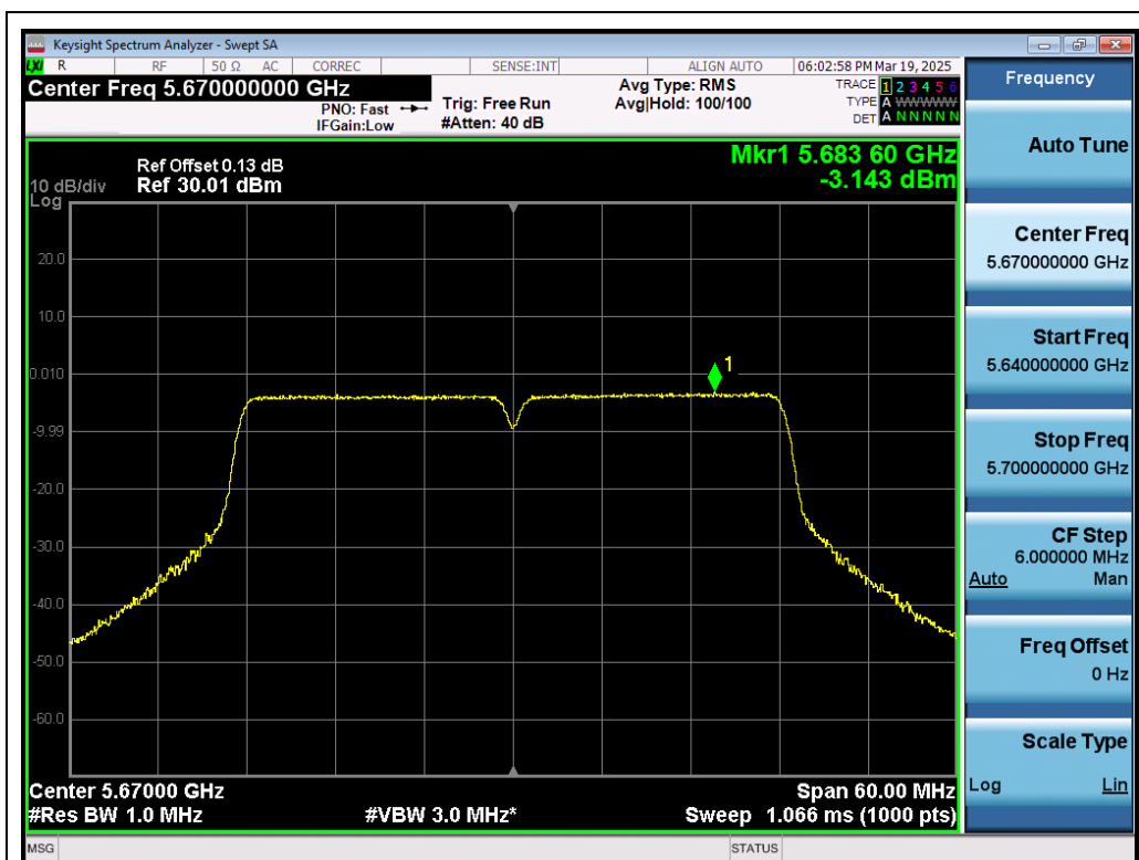
Test_Graph_802.11n40_ANT1_5670_MCS0_PSD
