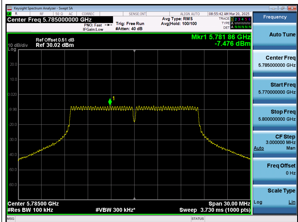
Test_Graph_802.11a_ANT1_5785_6Mbps_PSD
