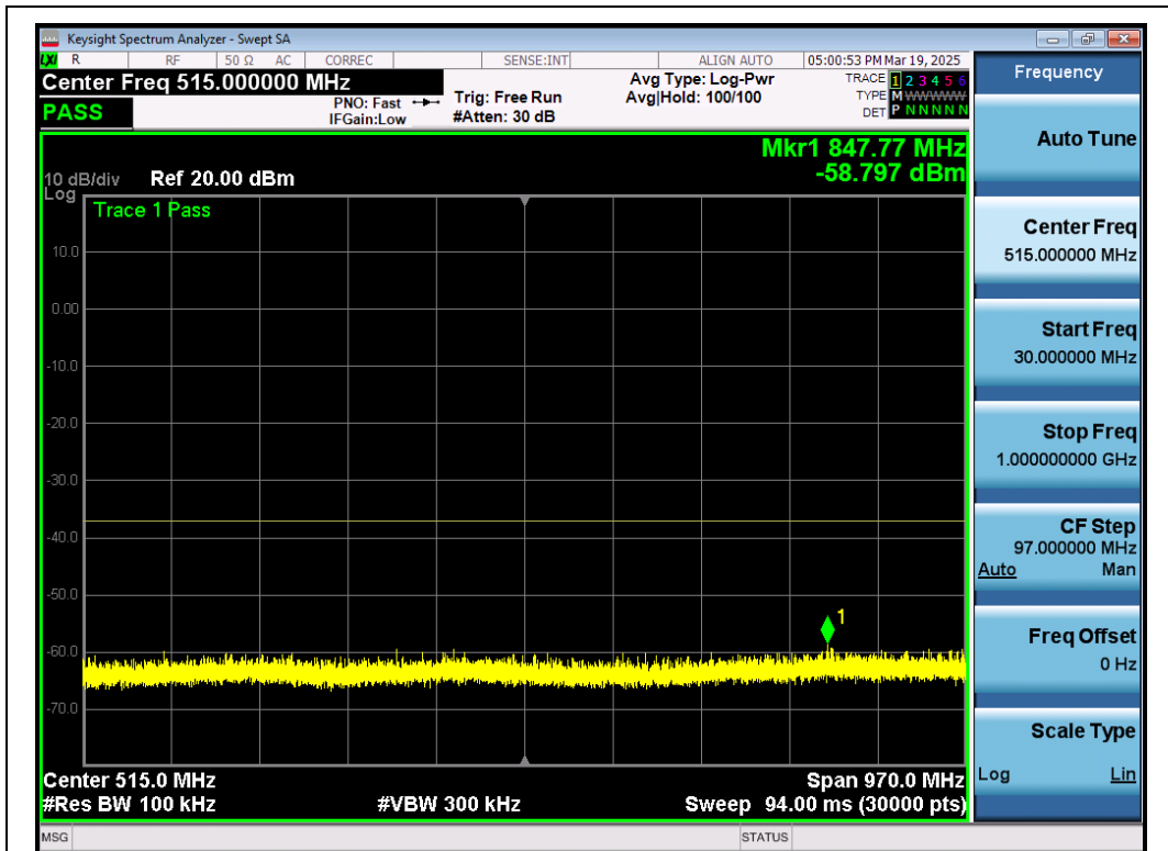
Test_Graph_802.11ac80_ANT1_5210_MCS0_Frequency Band 1
