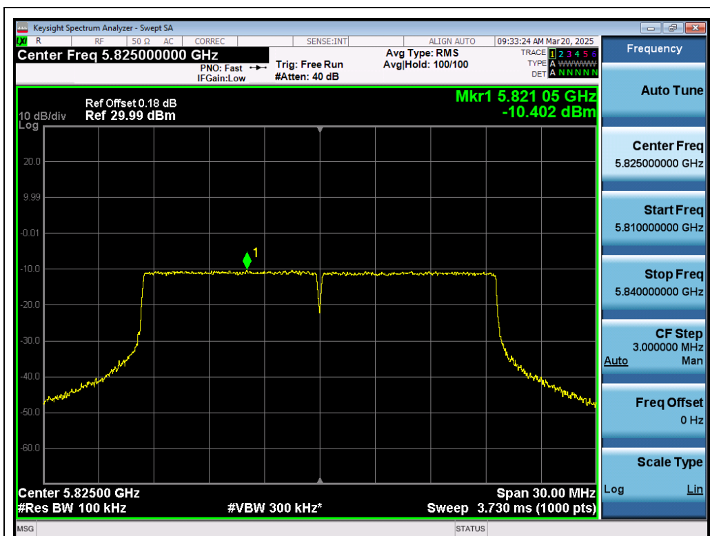
Test_Graph_802.11ax20_ANT1_5825_MCS0_PSD
