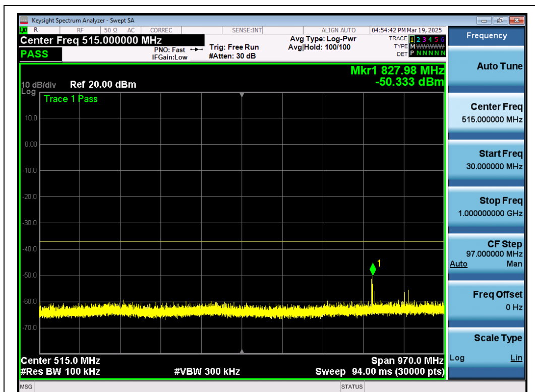
Test_Graph_802.11n40_ANT1_5230_MCS0_Frequency Band 1
