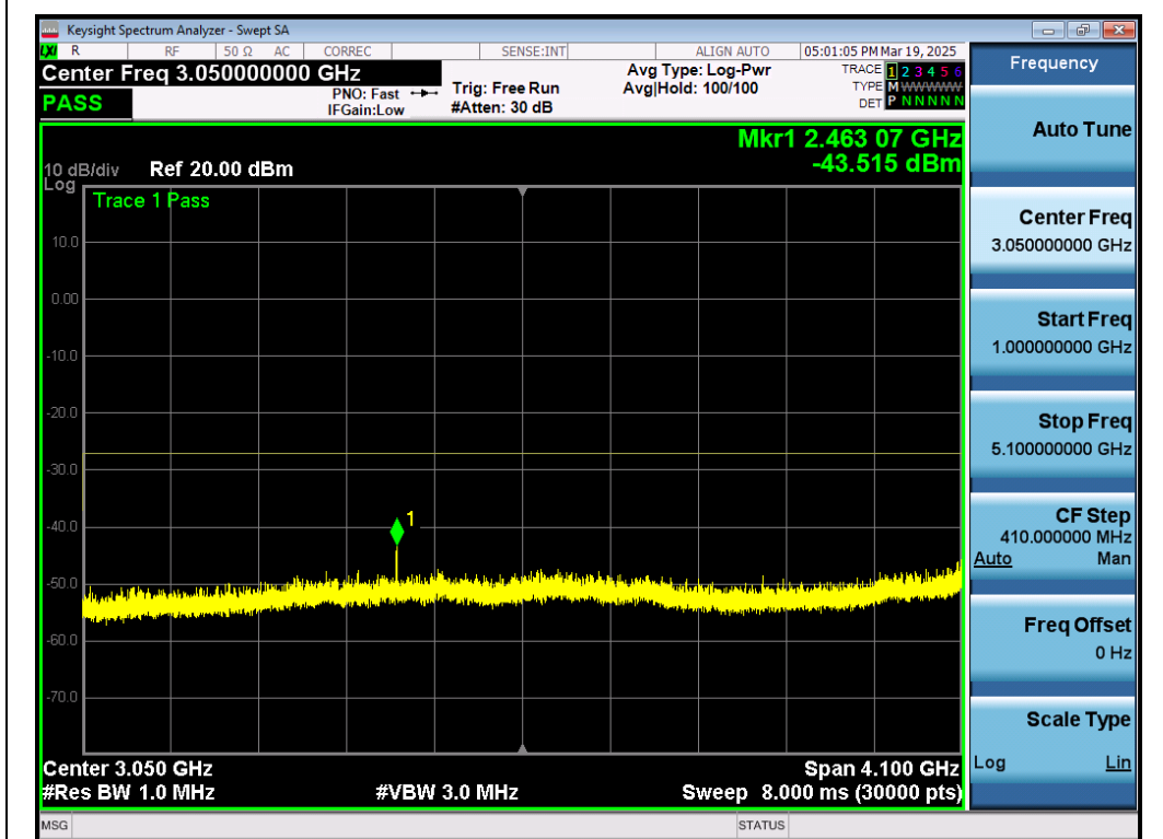
Test_Graph_802.11ac80_ANT1_5210_MCS0_Frequency Band 2
