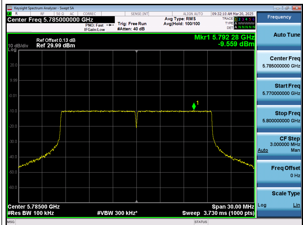
Test_Graph_802.11ax20_ANT1_5785_MCS0_PSD
