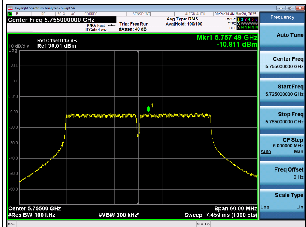
Test_Graph_802.11ac40_ANT1_5755_MCS0_PSD
