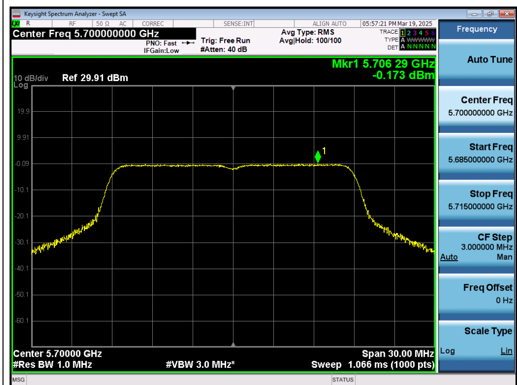
Test_Graph_802.11n20_ANT1_5700_MCS0_PSD
