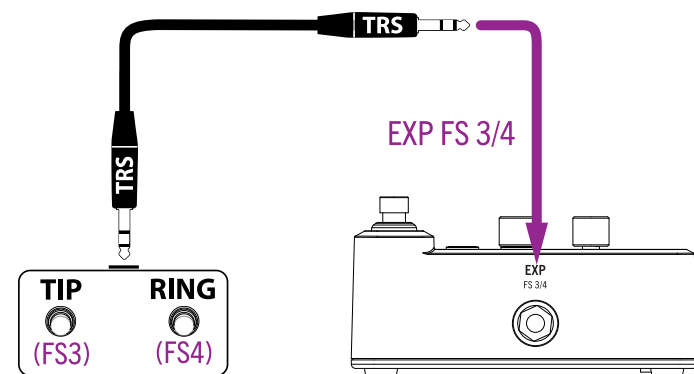
Connecting a dual-footswitch (TRS - TRS connection)
