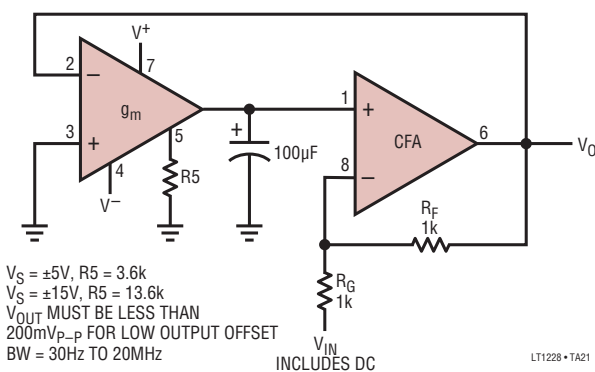
Inverting Amplifier with DC Output Less Than 5mV
