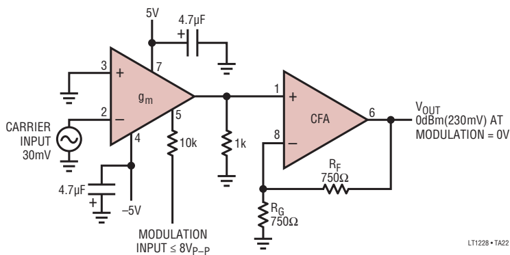
Amplitude Modulator
