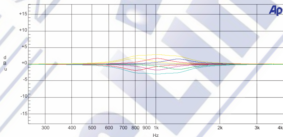
Figure 1 Symmetrical-Q equaliser "wide" mode \pm 2 dB boost and cut
