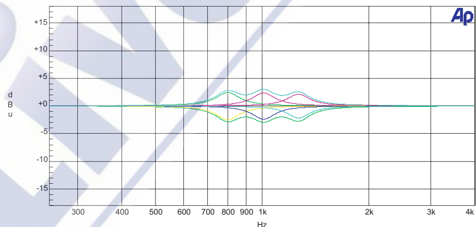
Figure 2 Symmetrical-Q equaliser "narrow" mode \pm 2 dB boost and cut
