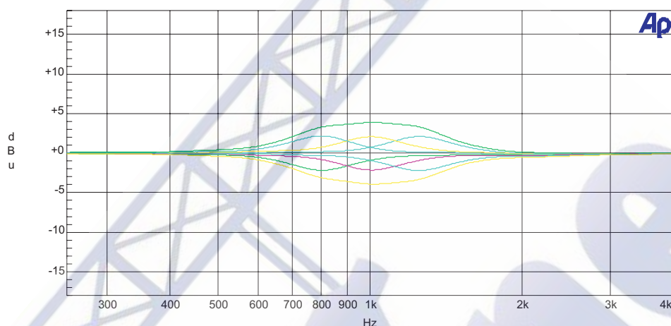
Figure 5 DN370 response \pm 2 dB boost and cut
