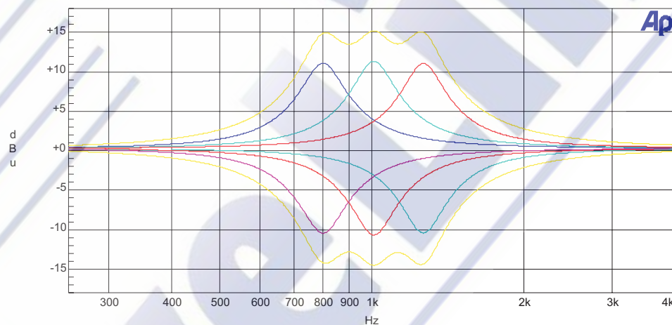
Figure 4 Symmetrical-Q equaliser "narrow" mode full boost and cut
