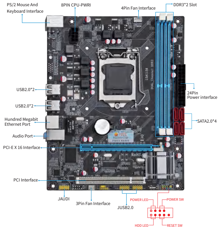
1-1 P55 motherboard illustration
