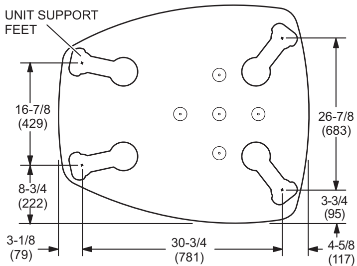
TOP VIEW BASE SECTION (Large Base)
