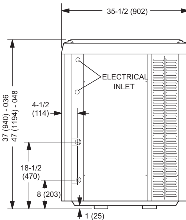
ACCESS VIEW
