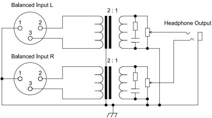
Fig 1-5: CM-HPX1 Block Diagram
