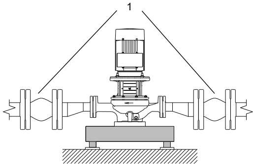
TP pump installed with larger expansion joints
