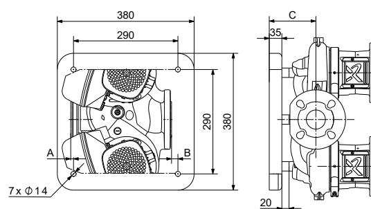
Drawing, TPE2 D, TPE3 D 80
