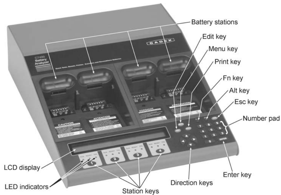
Figure 1: Top and front panel of C7400 & C7400ER battery analyzer
