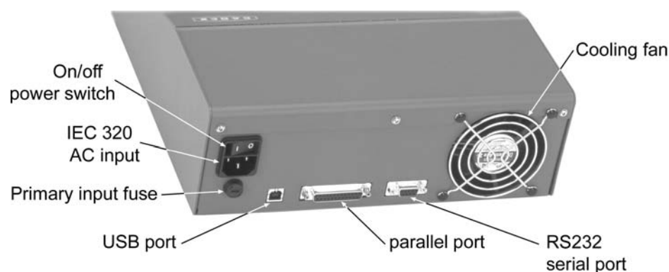
Figure 3: Rear panel of Cadex battery analyzer
