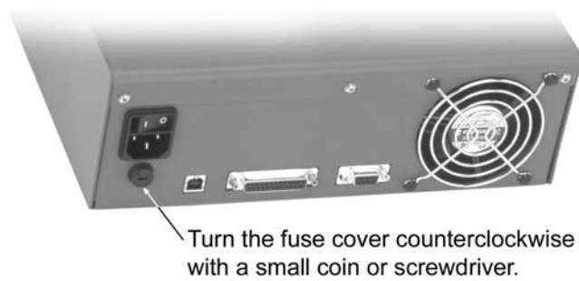
Figure 12: Replacing the fuse
