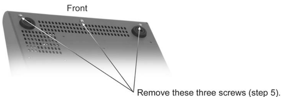
Figure 14: C7200: Remove the bottom screws
