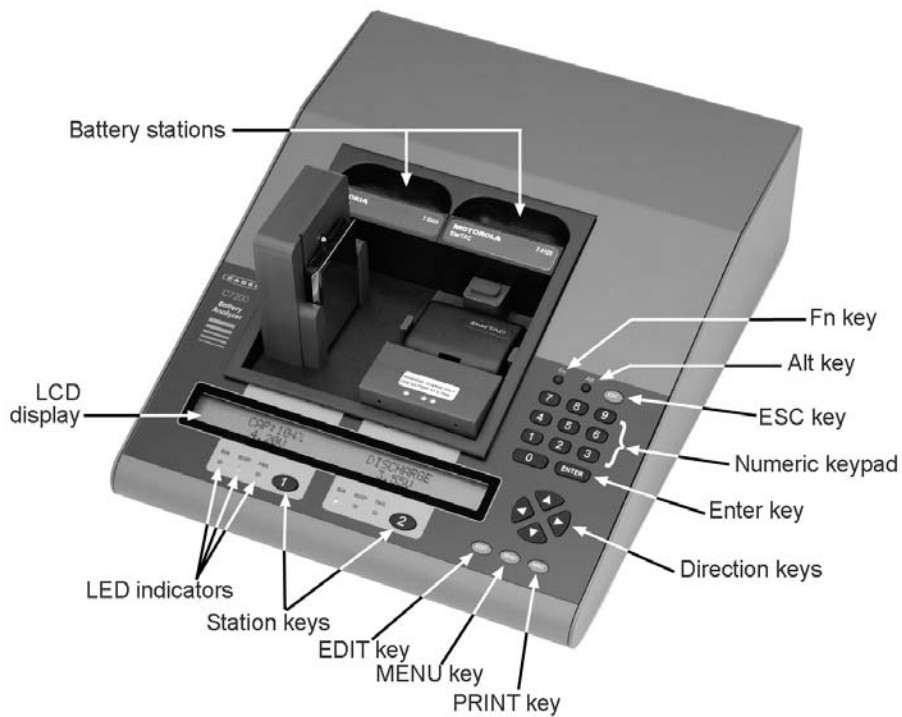
Figure 2: Top and front panel of Cadex C7200 Battery Analyzer
