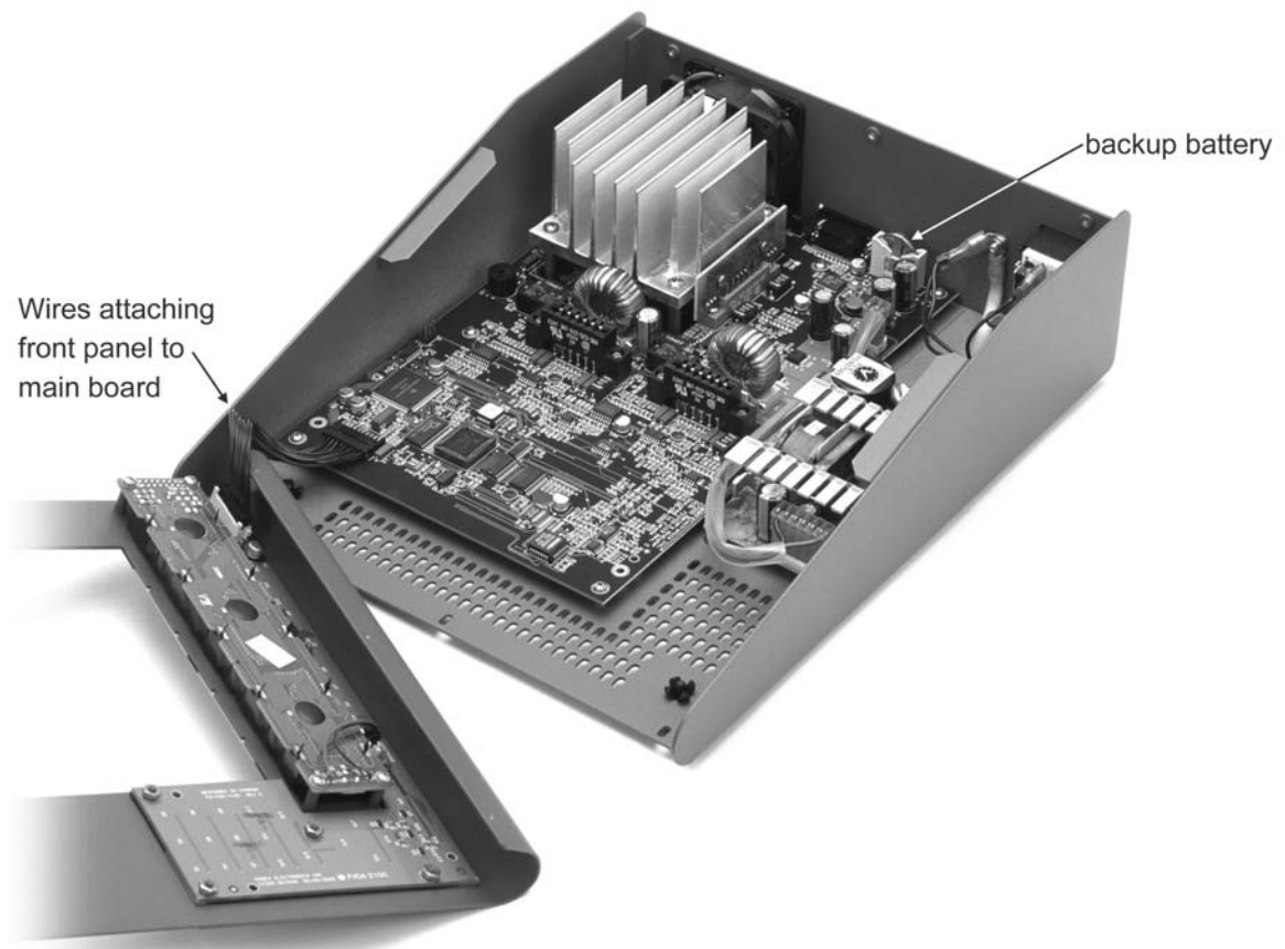
Figure 16: Cadex C7200 with cover removed
