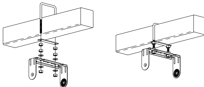
Figure 3.3: U-Bolt - 4-inch
