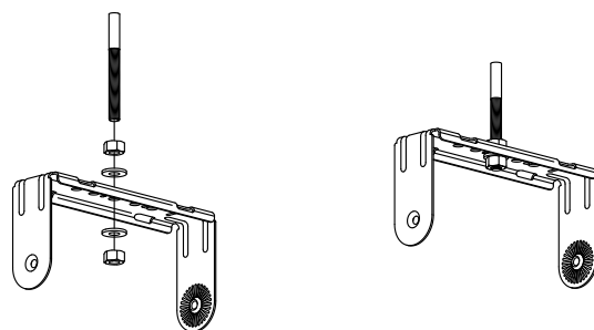
Figure 3.4: Threaded rod
