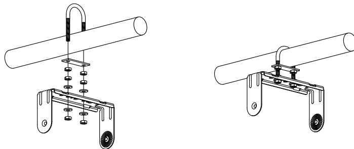
Figure 3.2: U-Bolt - 2-inch
