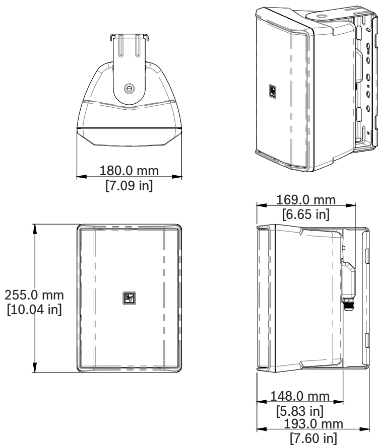
Figure 5.1: EVID-S5.2X dimensions
