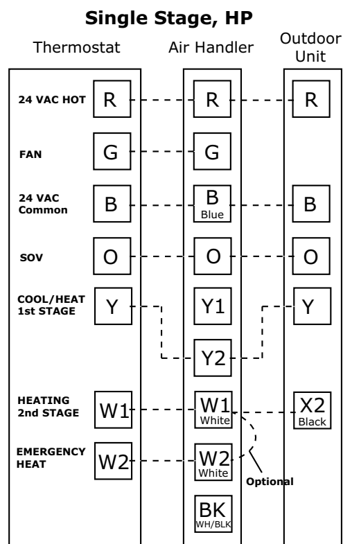
Figure 5. Field Wiring Diagram — A4AH6V — Single Stage
