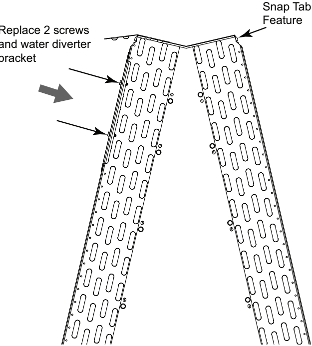
Figure 35. A4AH6E49, A4AH6E61, A4AH6V48, A4AH6V60 — Rear view
