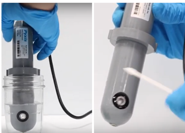
Figure 19. Cleaning of HM-500 Series Sensor
