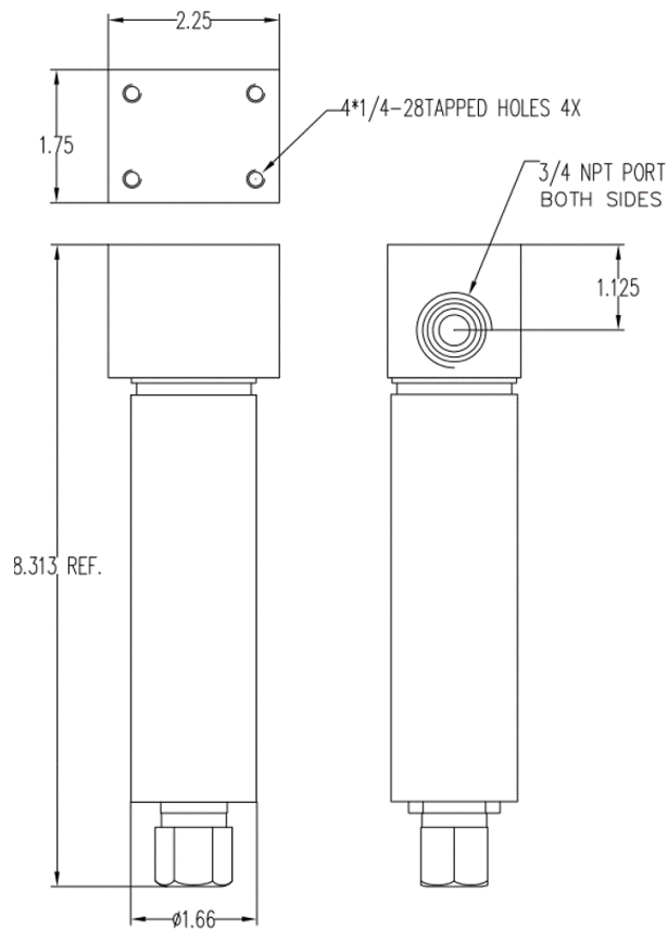
Figure 4. Dimension of the HM-500SS/510SS/520SS (inch)
