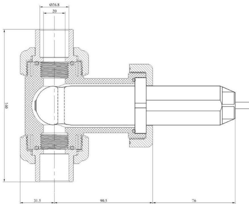
Figure 3. Dimension of the HM-500/510/520 sensor and the ST-001 Tee Assembly (mm)
