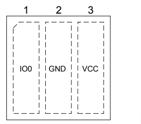
Figure 4. DFN3 pinout - Top view
