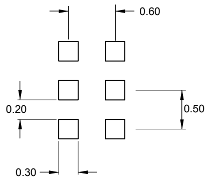
Figure 34. X2F-PSON6 - Footprint example
