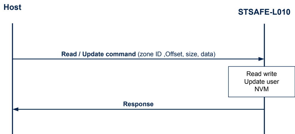
Figure 5. STSAFE-L010 data read/update sequence
