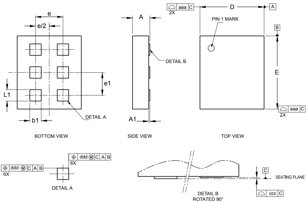
Figure 33. X2F-PS0N6 - Outline
