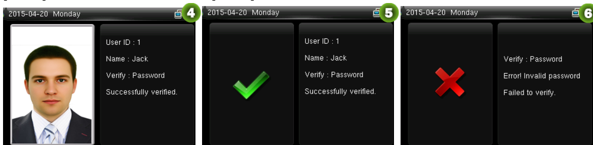
Verification succeeds
