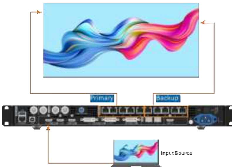
Figure 5-28 Ethernet port backup connection
