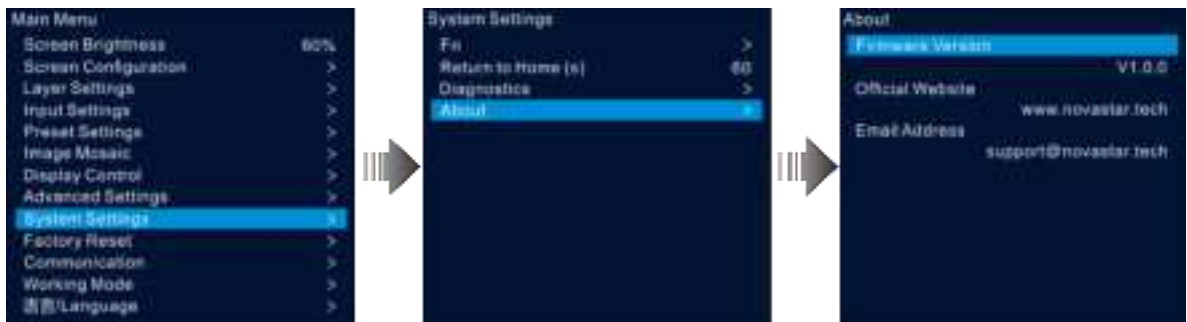
Figure 5-47 About
