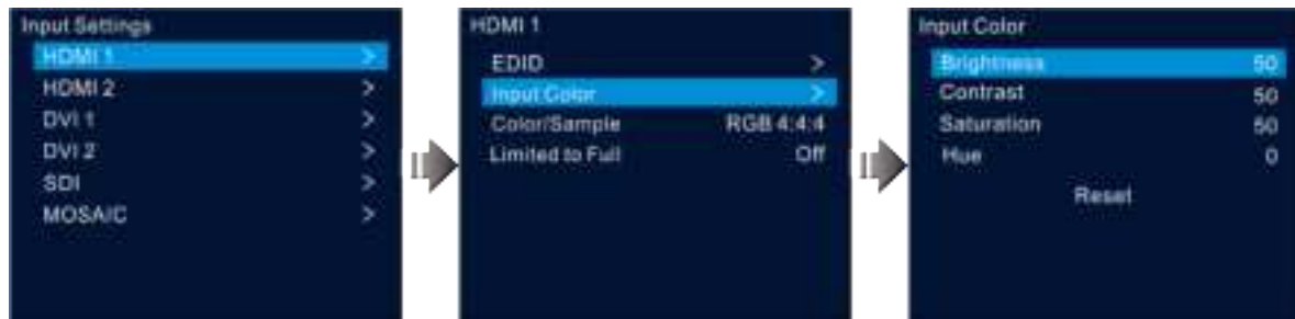
Figure 5-20 Input color
