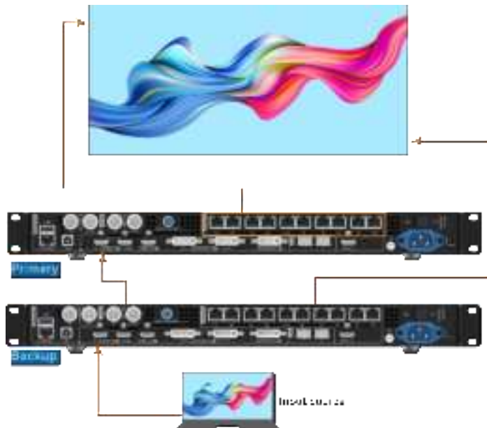
Figure 5-26 Device backup connection
