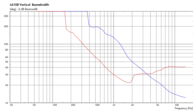
LA108 Vertical beamwidth
