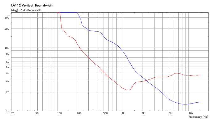
LA112 Vertical beamwidth
