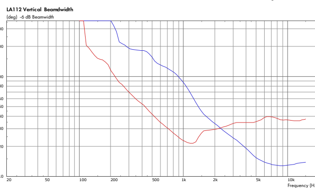
LA112 Vertical beamwidth Single-box (blue). Three-boxes set at 12 deg splay angles (red).
