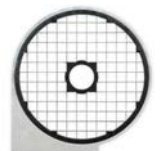
14x14x14 mm Code: 321012-DR140 (Only work in VC65MS with SA014)
