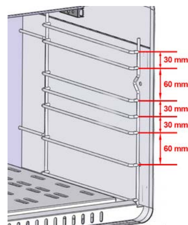
YSD-6A Level Distance
