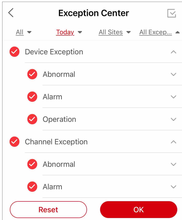
Figure 9-3 Exception Types
