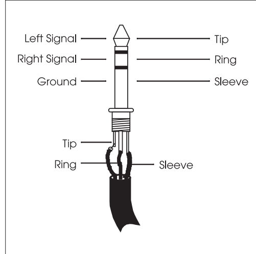
1/4" Headphones Connector
