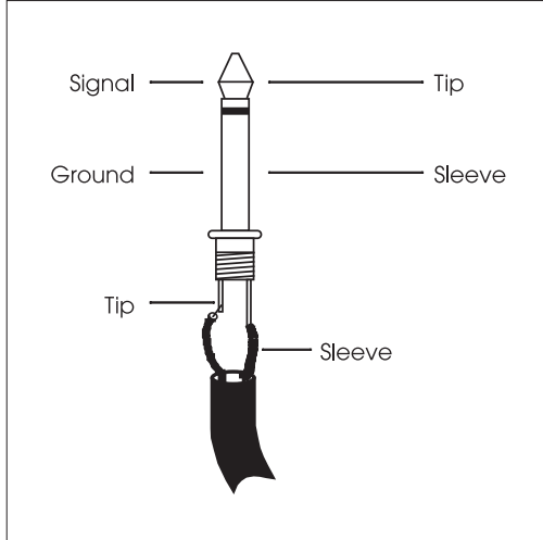
1/4" Audio Connector
