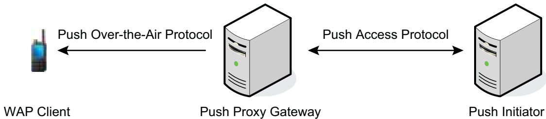
Figure 19: Push Framework
